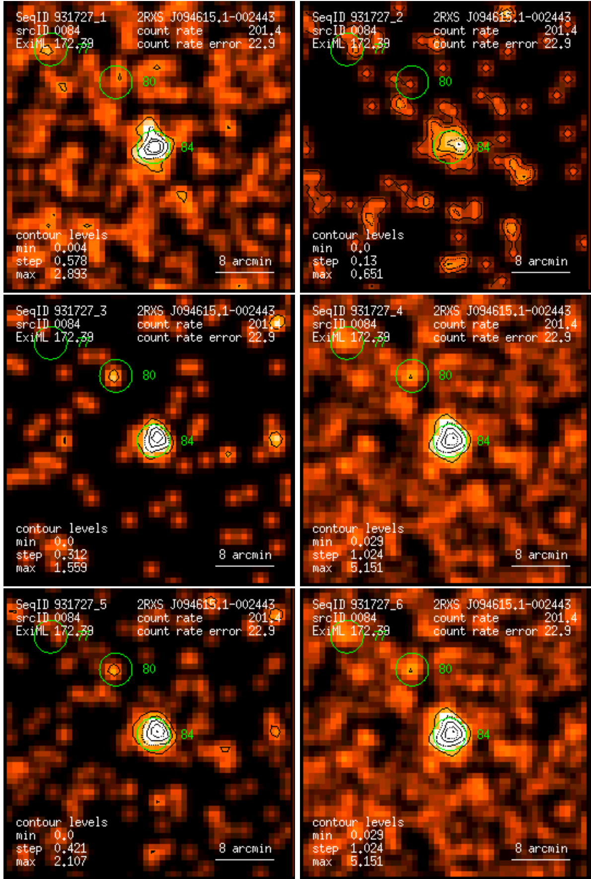
Figure 84: RASS 931727: detection 0084: band rate images, Gaussian filter: (1) PSPC channels 11 – 41, (2) 52 – 90, (3) 91 – 201, (4) 11 – 235, (5) 52 – 201, (6) 11 – 201. Broad band rates in counts/ks. Band rate contour levels in counts/ks/arcmin 2 .
