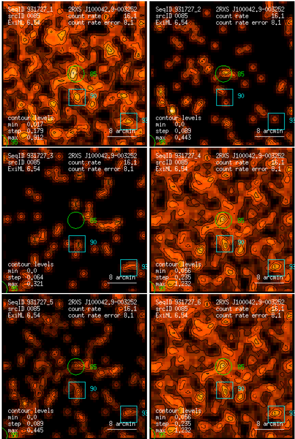
Figure 85: RASS 931727: detection 0085: band rate images, Gaussian filter: (1) PSPC channels 11 – 41, (2) 52 – 90, (3) 91 – 201, (4) 11 – 235, (5) 52 – 201, (6) 11 – 201. Broad band rates in counts/ks. Band rate contour levels in counts/ks/arcmin 2 .
