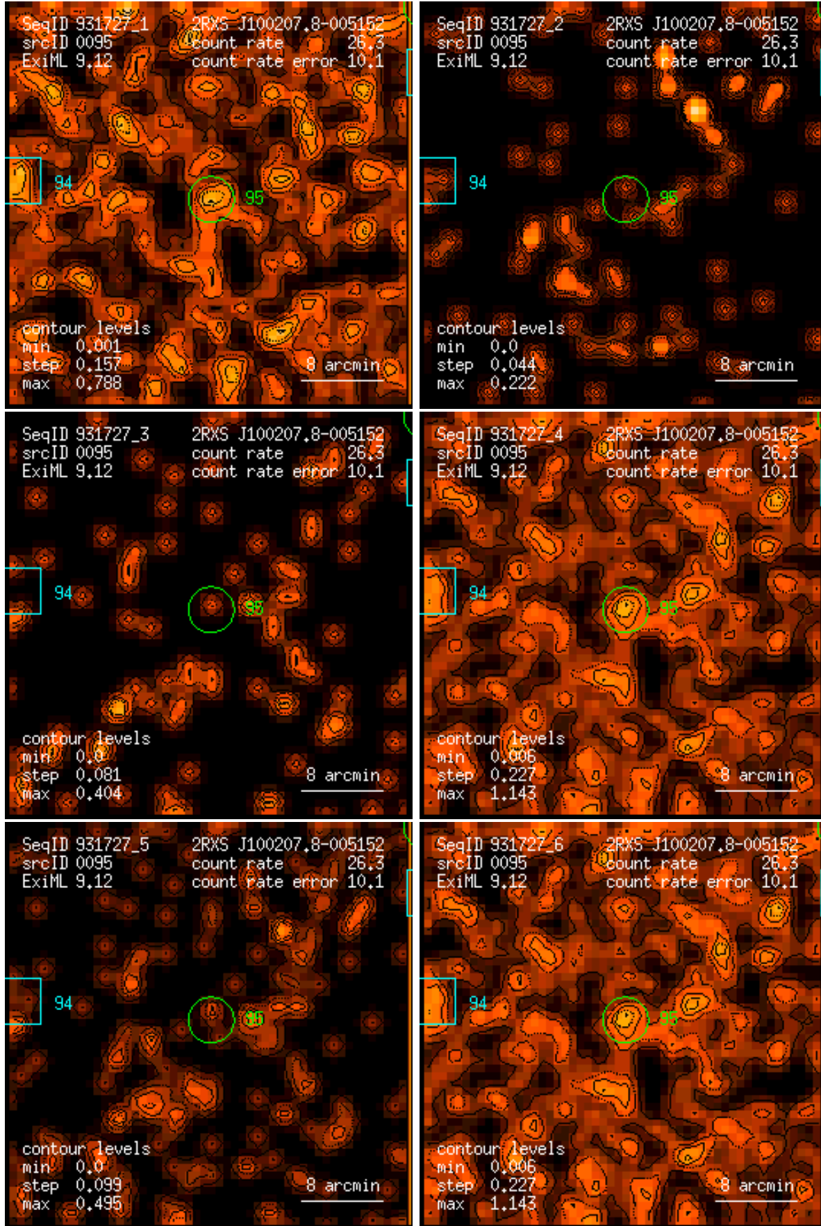
Figure 95: RASS 931727: detection 0095: band rate images, Gaussian filter: (1) PSPC channels 11 – 41, (2) 52 – 90, (3) 91 – 201, (4) 11 – 235, (5) 52 – 201, (6) 11 – 201. Broad band rates in counts/ks. Band rate contour levels in counts/ks/arcmin 2 .
