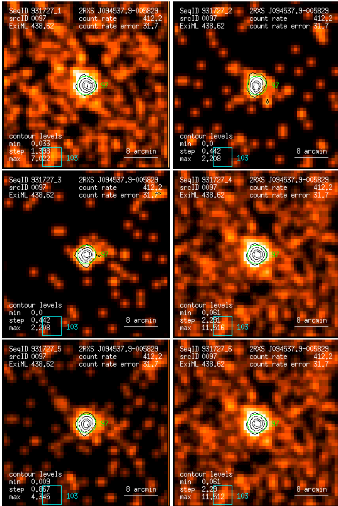
Figure 97: RASS 931727: detection 0097: band rate images, Gaussian filter: (1) PSPC channels 11 – 41, (2) 52 – 90, (3) 91 – 201, (4) 11 – 235, (5) 52 – 201, (6) 11 – 201. Broad band rates in counts/ks. Band rate contour levels in counts/ks/arcmin 2 .
