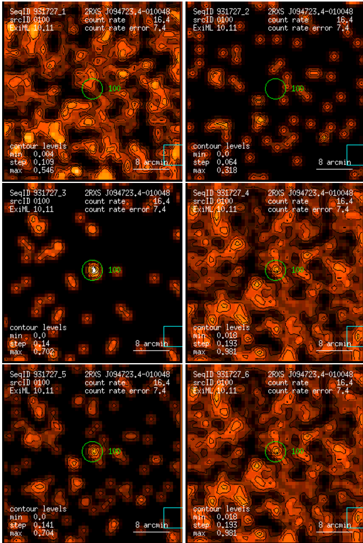
Figure 100: RASS 931727: detection 0100: band rate images, Gaussian filter: (1) PSPC channels 11 – 41, (2) 52 – 90, (3) 91 – 201, (4) 11 – 235, (5) 52 – 201, (6) 11 – 201. Broad band rates in counts/ks. Band rate contour levels in counts/ks/arcmin 2 .
