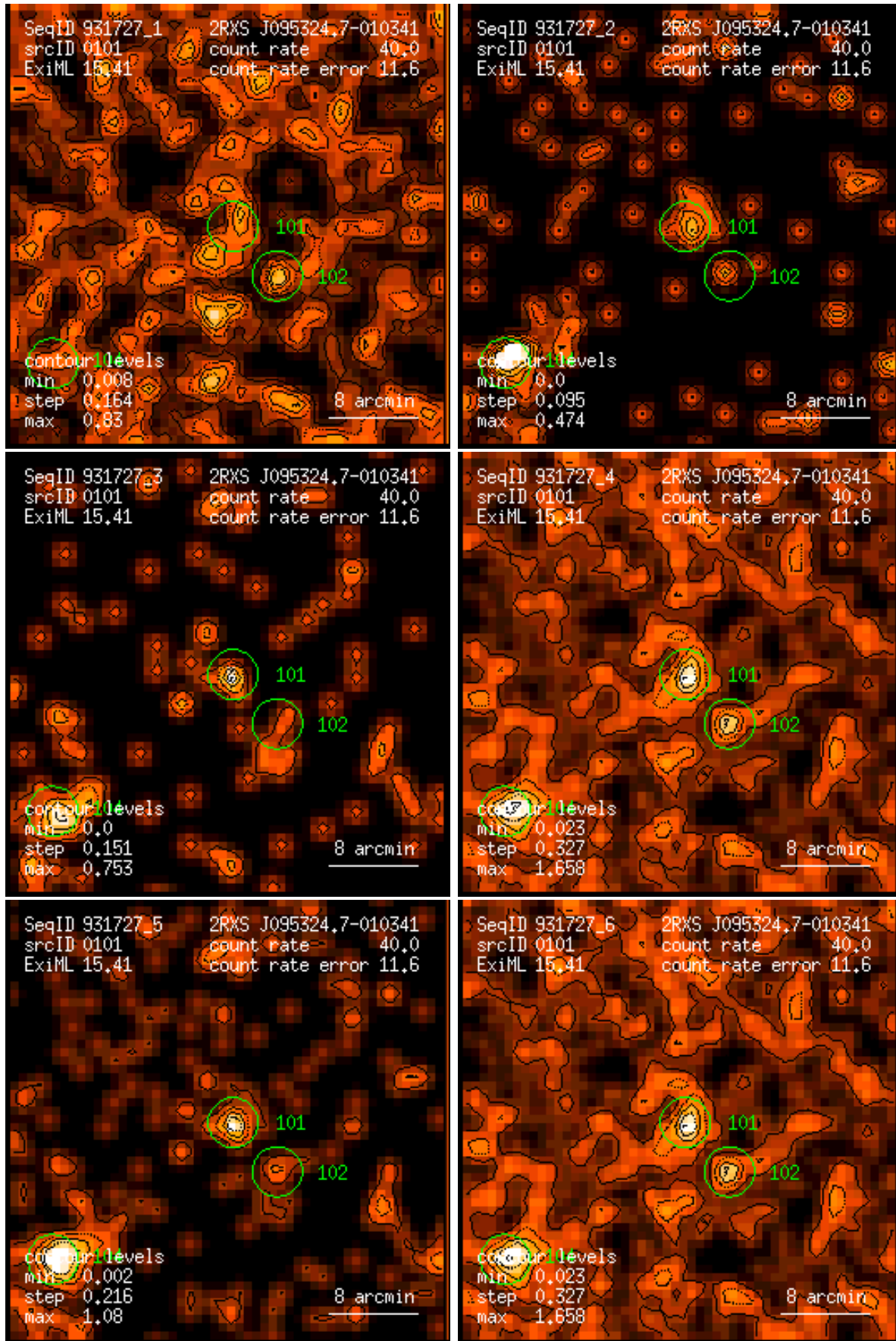
Figure 101: RASS 931727: detection 0101: band rate images, Gaussian filter: (1) PSPC channels 11 – 41, (2) 52 – 90, (3) 91 – 201, (4) 11 – 235, (5) 52 – 201, (6) 11 – 201. Broad band rates in counts/ks. Band rate contour levels in counts/ks/arcmin 2 .
