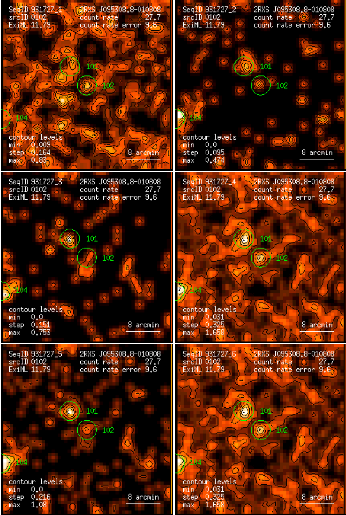
Figure 102: RASS 931727: detection 0102: band rate images, Gaussian filter: (1) PSPC channels 11 – 41, (2) 52 – 90, (3) 91 – 201, (4) 11 – 235, (5) 52 – 201, (6) 11 – 201. Broad band rates in counts/ks. Band rate contour levels in counts/ks/arcmin 2 .
