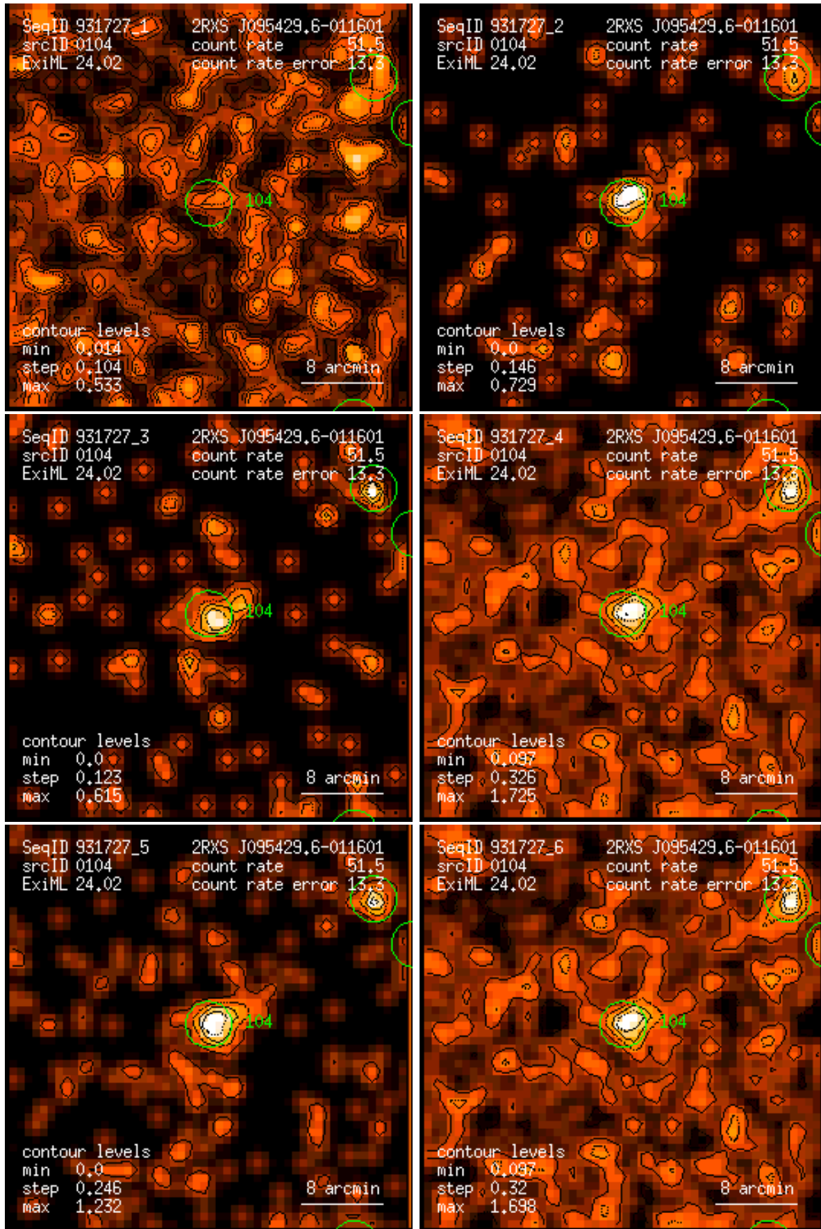
Figure 104: RASS 931727: detection 0104: band rate images, Gaussian filter: (1) PSPC channels 11 – 41, (2) 52 – 90, (3) 91 – 201, (4) 11 – 235, (5) 52 – 201, (6) 11 – 201. Broad band rates in counts/ks. Band rate contour levels in counts/ks/arcmin 2 .
