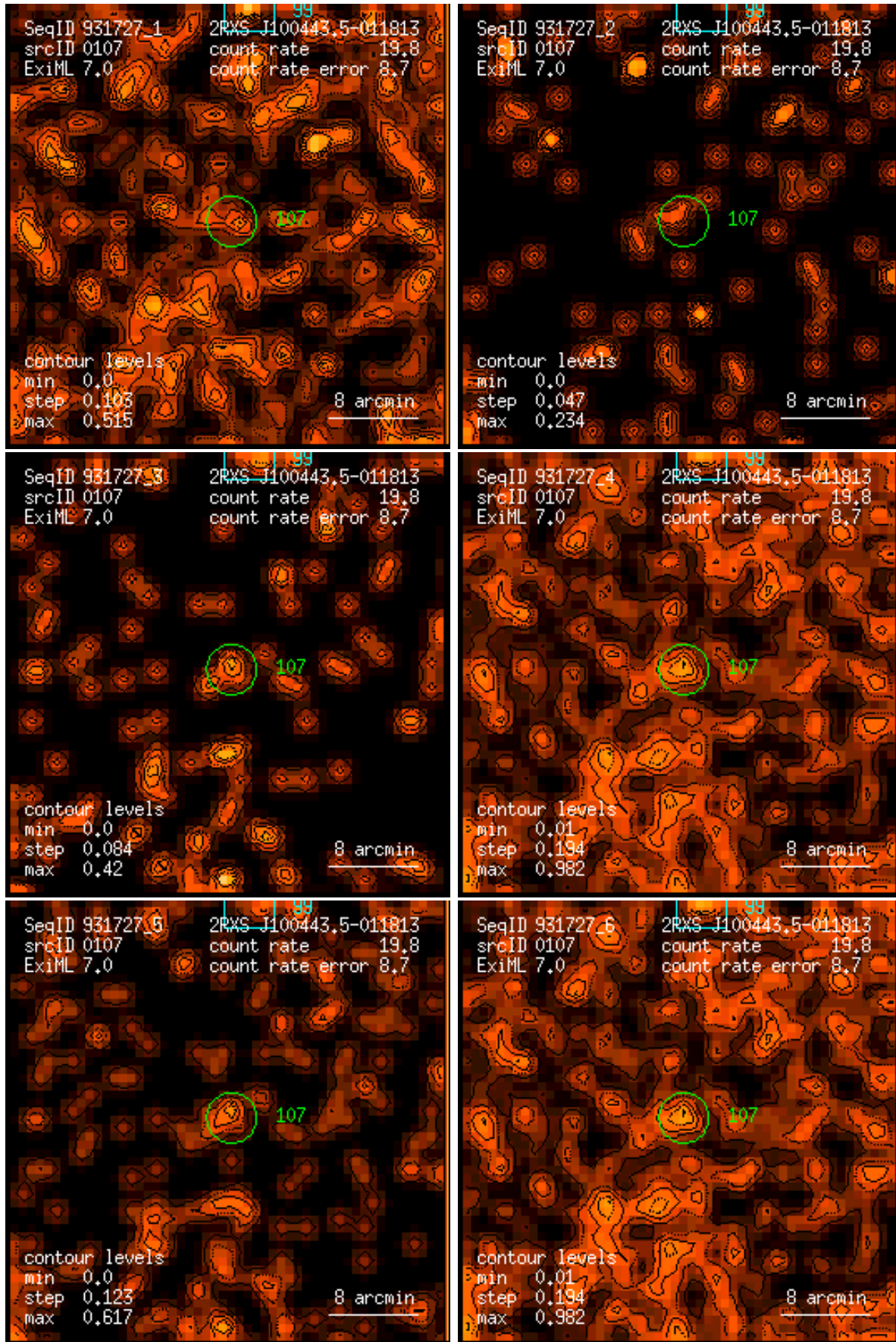
Figure 107: RASS 931727: detection 0107: band rate images, Gaussian filter: (1) PSPC channels 11 – 41, (2) 52 – 90, (3) 91 – 201, (4) 11 – 235, (5) 52 – 201, (6) 11 – 201. Broad band rates in counts/ks. Band rate contour levels in counts/ks/arcmin 2 .
