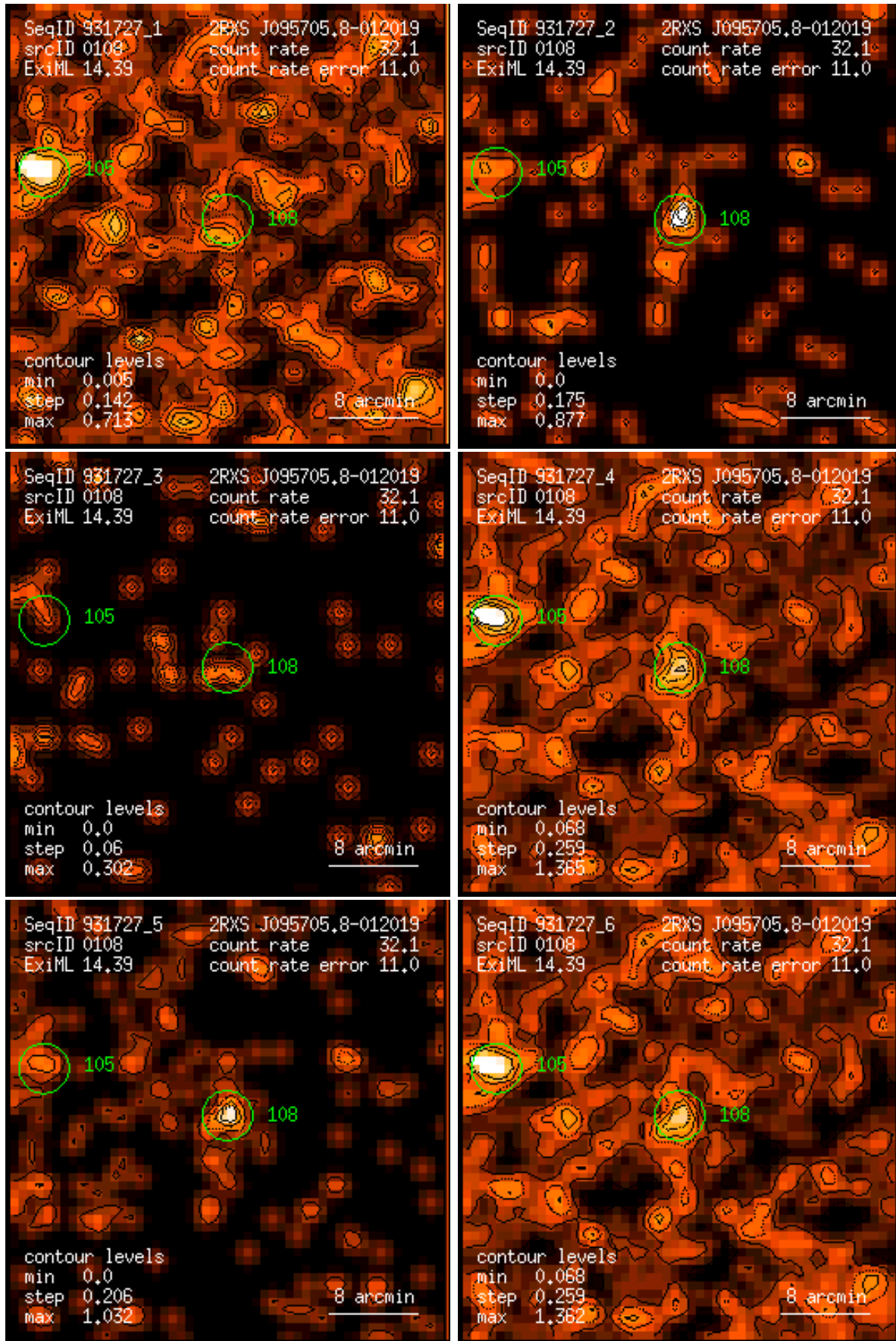
Figure 108: RASS 931727: detection 0108: band rate images, Gaussian filter: (1) PSPC channels 11 – 41, (2) 52 – 90, (3) 91 – 201, (4) 11 – 235, (5) 52 – 201, (6) 11 – 201. Broad band rates in counts/ks. Band rate contour levels in counts/ks/arcmin 2 .
