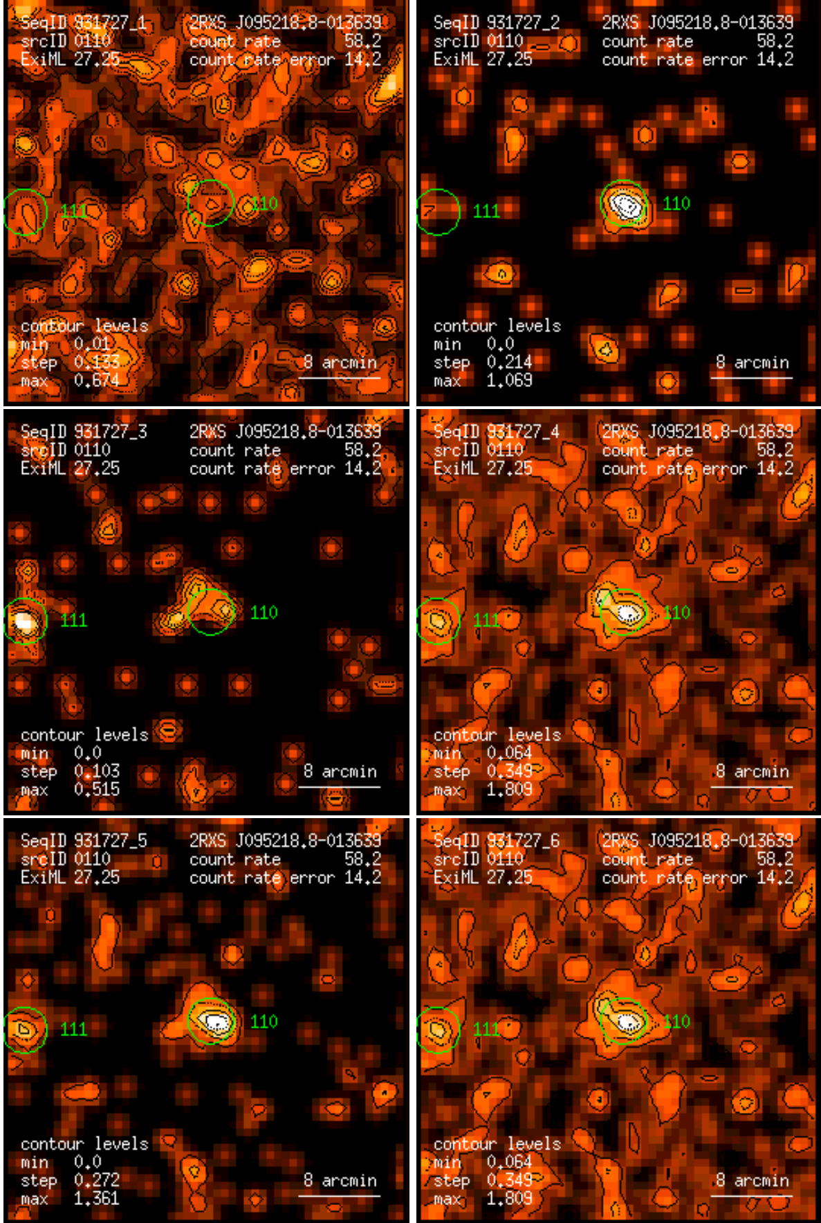
Figure 110: RASS 931727: detection 0110: band rate images, Gaussian filter: (1) PSPC channels 11 – 41, (2) 52 – 90, (3) 91 – 201, (4) 11 – 235, (5) 52 – 201, (6) 11 – 201. Broad band rates in counts/ks. Band rate contour levels in counts/ks/arcmin 2 .
