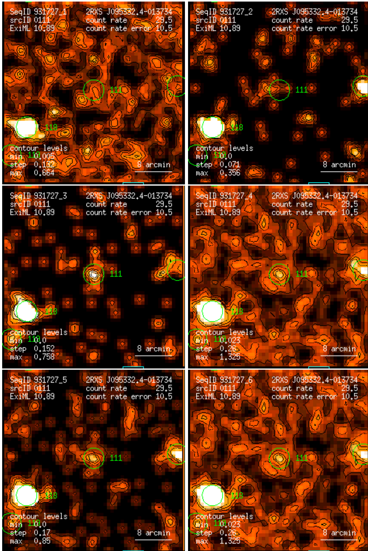
Figure 111: RASS 931727: detection 0111: band rate images, Gaussian filter: (1) PSPC channels 11 – 41, (2) 52 – 90, (3) 91 – 201, (4) 11 – 235, (5) 52 – 201, (6) 11 – 201. Broad band rates in counts/ks. Band rate contour levels in counts/ks/arcmin 2 .
