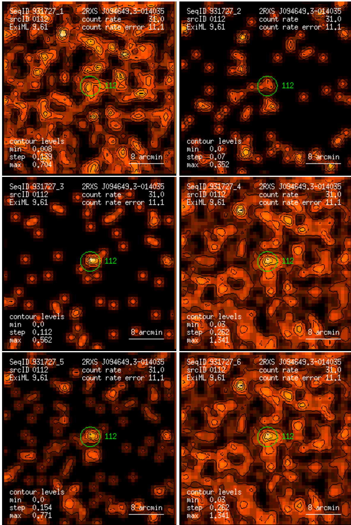
Figure 112: RASS 931727: detection 0112: band rate images, Gaussian filter: (1) PSPC channels 11 – 41, (2) 52 – 90, (3) 91 – 201, (4) 11 – 235, (5) 52 – 201, (6) 11 – 201. Broad band rates in counts/ks. Band rate contour levels in counts/ks/arcmin 2 .
