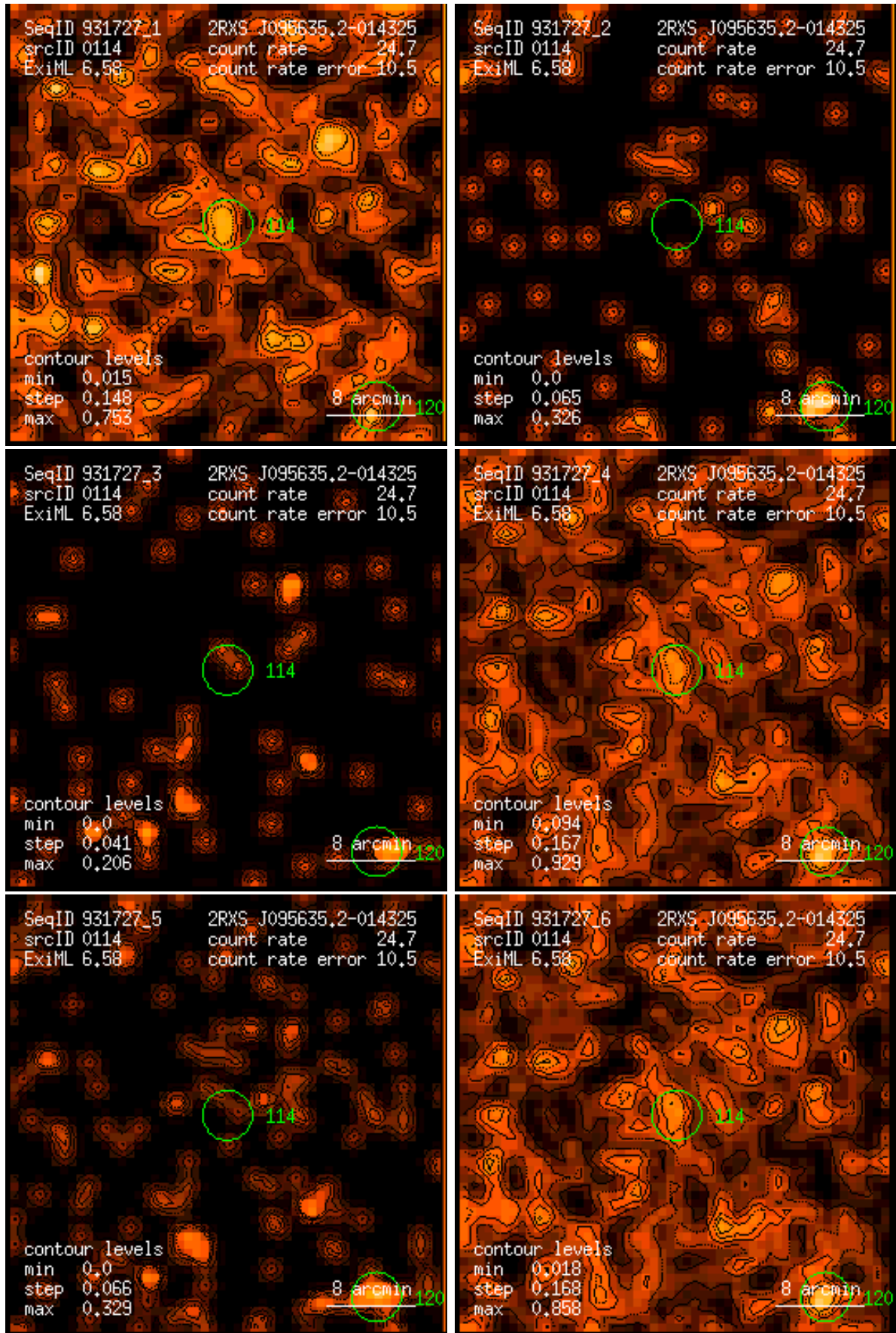
Figure 114: RASS 931727: detection 0114: band rate images, Gaussian filter: (1) PSPC channels 11 – 41, (2) 52 – 90, (3) 91 – 201, (4) 11 – 235, (5) 52 – 201, (6) 11 – 201. Broad band rates in counts/ks. Band rate contour levels in counts/ks/arcmin 2 .
