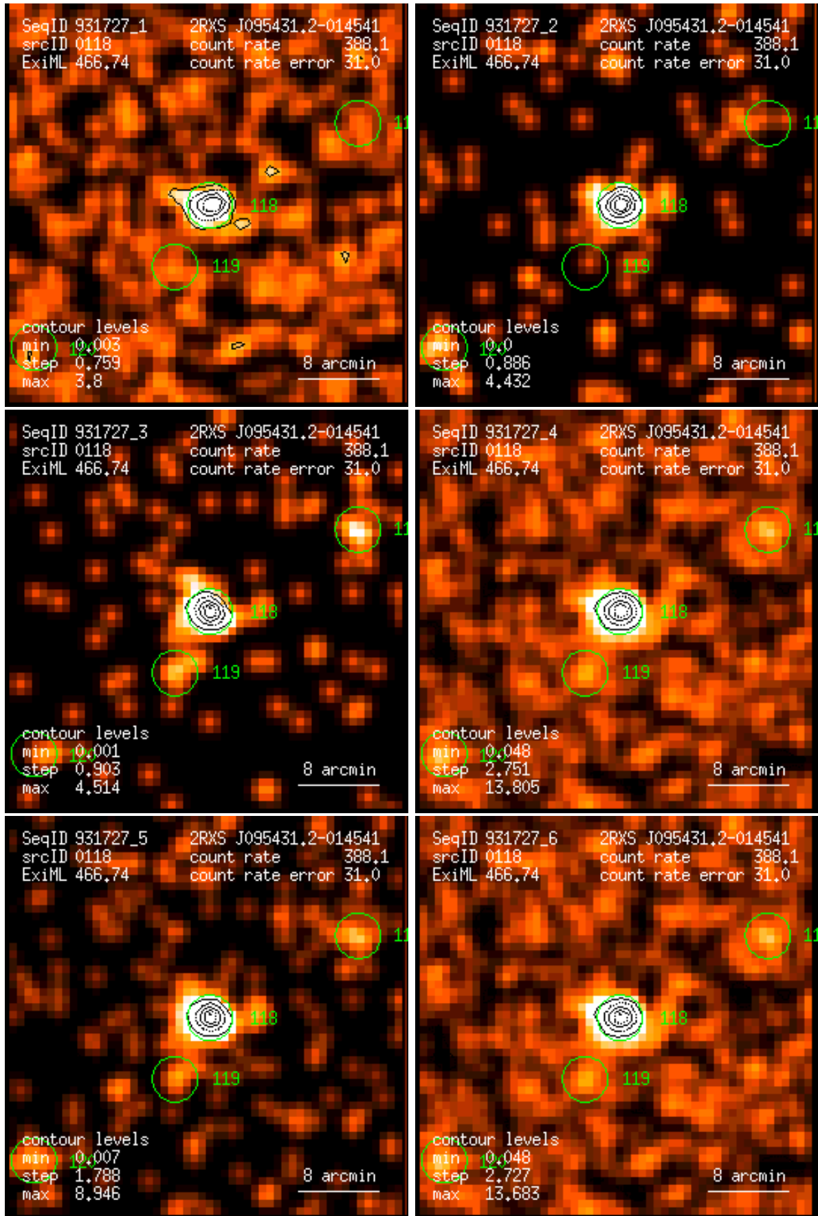
Figure 118: RASS 931727: detection 0118: band rate images, Gaussian filter: (1) PSPC channels 11 – 41, (2) 52 – 90, (3) 91 – 201, (4) 11 – 235, (5) 52 – 201, (6) 11 – 201. Broad band rates in counts/ks. Band rate contour levels in counts/ks/arcmin 2 .
