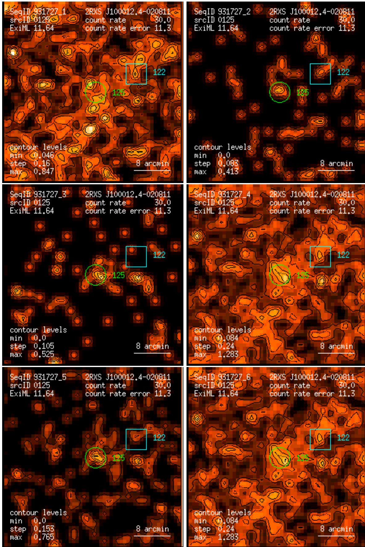
Figure 125: RASS 931727: detection 0125: band rate images, Gaussian filter: (1) PSPC channels 11 – 41, (2) 52 – 90, (3) 91 – 201, (4) 11 – 235, (5) 52 – 201, (6) 11 – 201. Broad band rates in counts/ks. Band rate contour levels in counts/ks/arcmin 2 .
