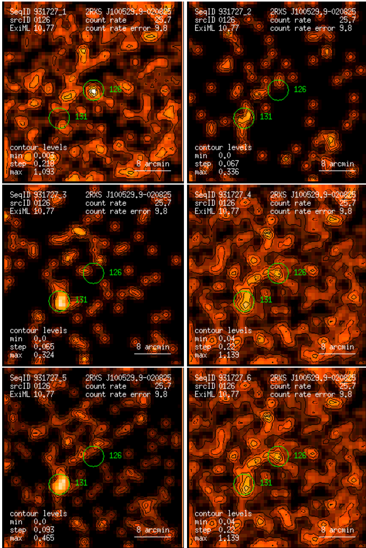
Figure 126: RASS 931727: detection 0126: band rate images, Gaussian filter: (1) PSPC channels 11 – 41, (2) 52 – 90, (3) 91 – 201, (4) 11 – 235, (5) 52 – 201, (6) 11 – 201. Broad band rates in counts/ks. Band rate contour levels in counts/ks/arcmin 2 .
