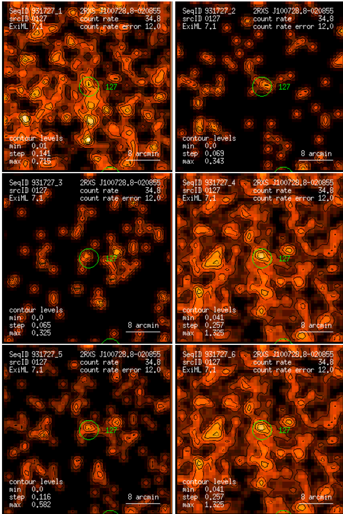
Figure 127: RASS 931727: detection 0127: band rate images, Gaussian filter: (1) PSPC channels 11 – 41, (2) 52 – 90, (3) 91 – 201, (4) 11 – 235, (5) 52 – 201, (6) 11 – 201. Broad band rates in counts/ks. Band rate contour levels in counts/ks/arcmin 2 .
