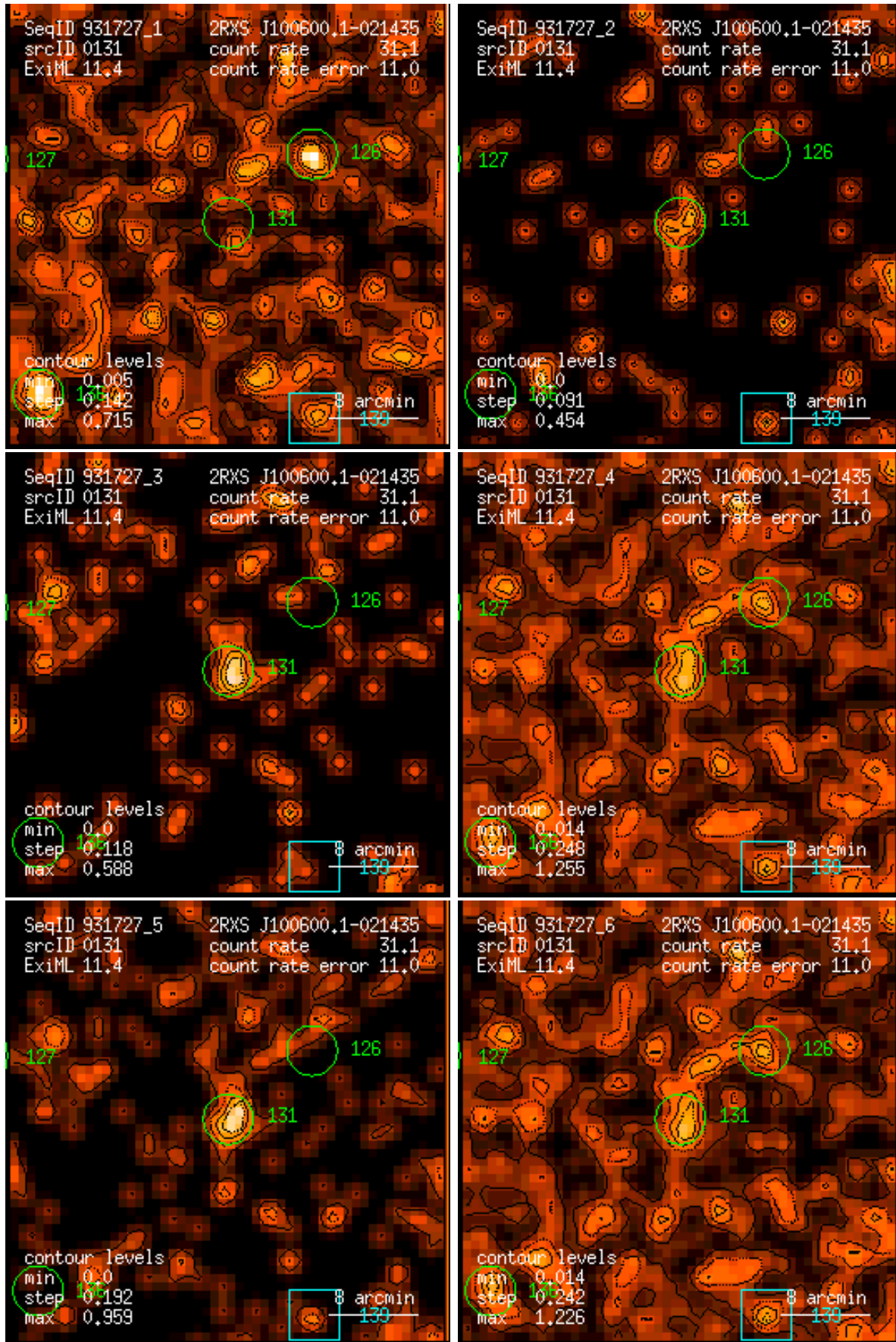
Figure 131: RASS 931727: detection 0131: band rate images, Gaussian filter: (1) PSPC channels 11 – 41, (2) 52 – 90, (3) 91 – 201, (4) 11 – 235, (5) 52 – 201, (6) 11 – 201. Broad band rates in counts/ks. Band rate contour levels in counts/ks/arcmin 2 .
