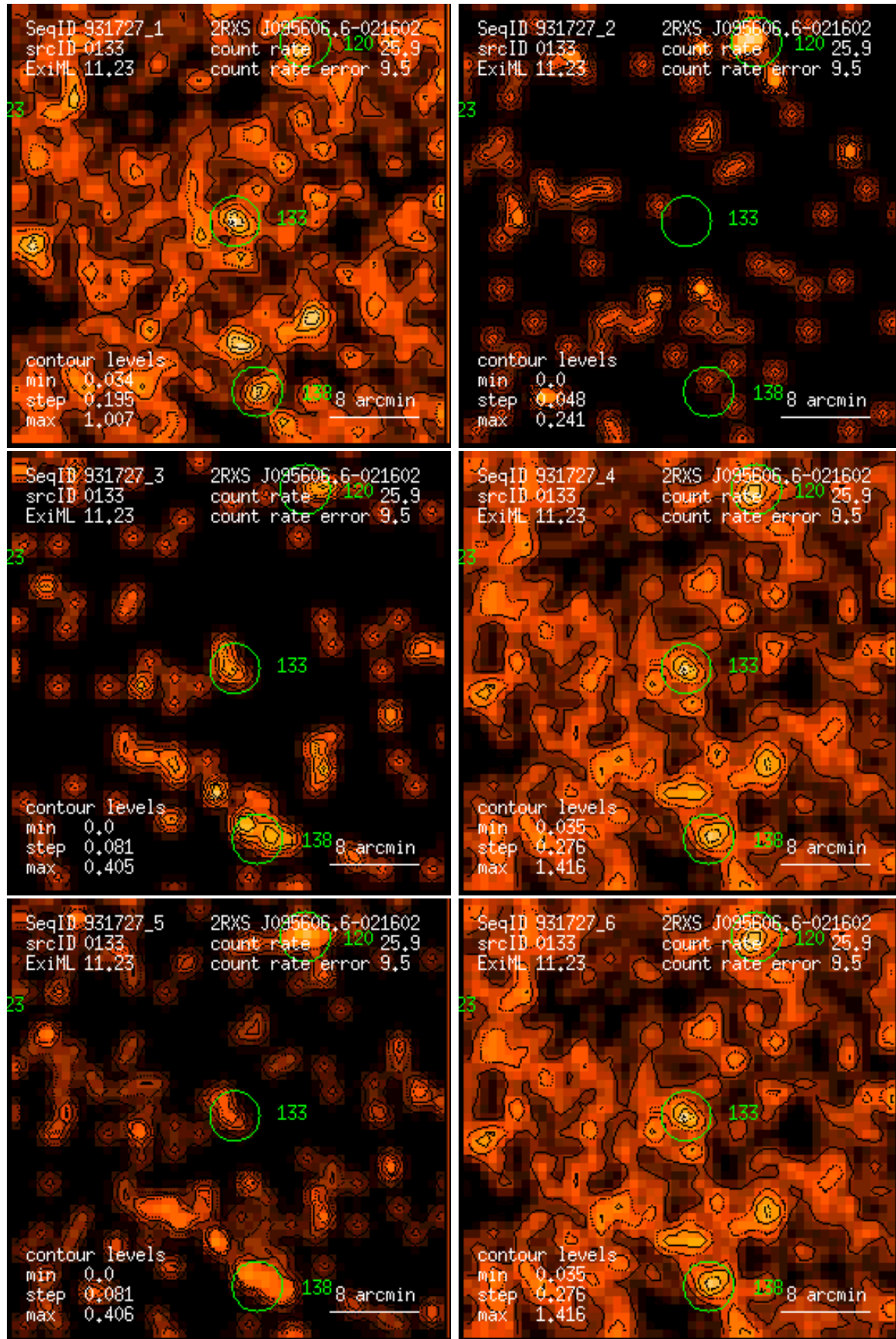
Figure 133: RASS 931727: detection 0133: band rate images, Gaussian filter: (1) PSPC channels 11 – 41, (2) 52 – 90, (3) 91 – 201, (4) 11 – 235, (5) 52 – 201, (6) 11 – 201. Broad band rates in counts/ks. Band rate contour levels in counts/ks/arcmin 2 .
