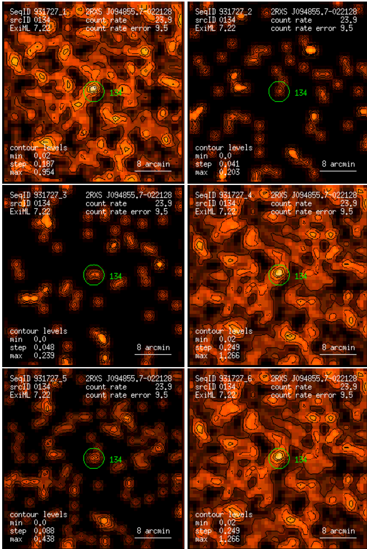
Figure 134: RASS 931727: detection 0134: band rate images, Gaussian filter: (1) PSPC channels 11 – 41, (2) 52 – 90, (3) 91 – 201, (4) 11 – 235, (5) 52 – 201, (6) 11 – 201. Broad band rates in counts/ks. Band rate contour levels in counts/ks/arcmin 2 .
