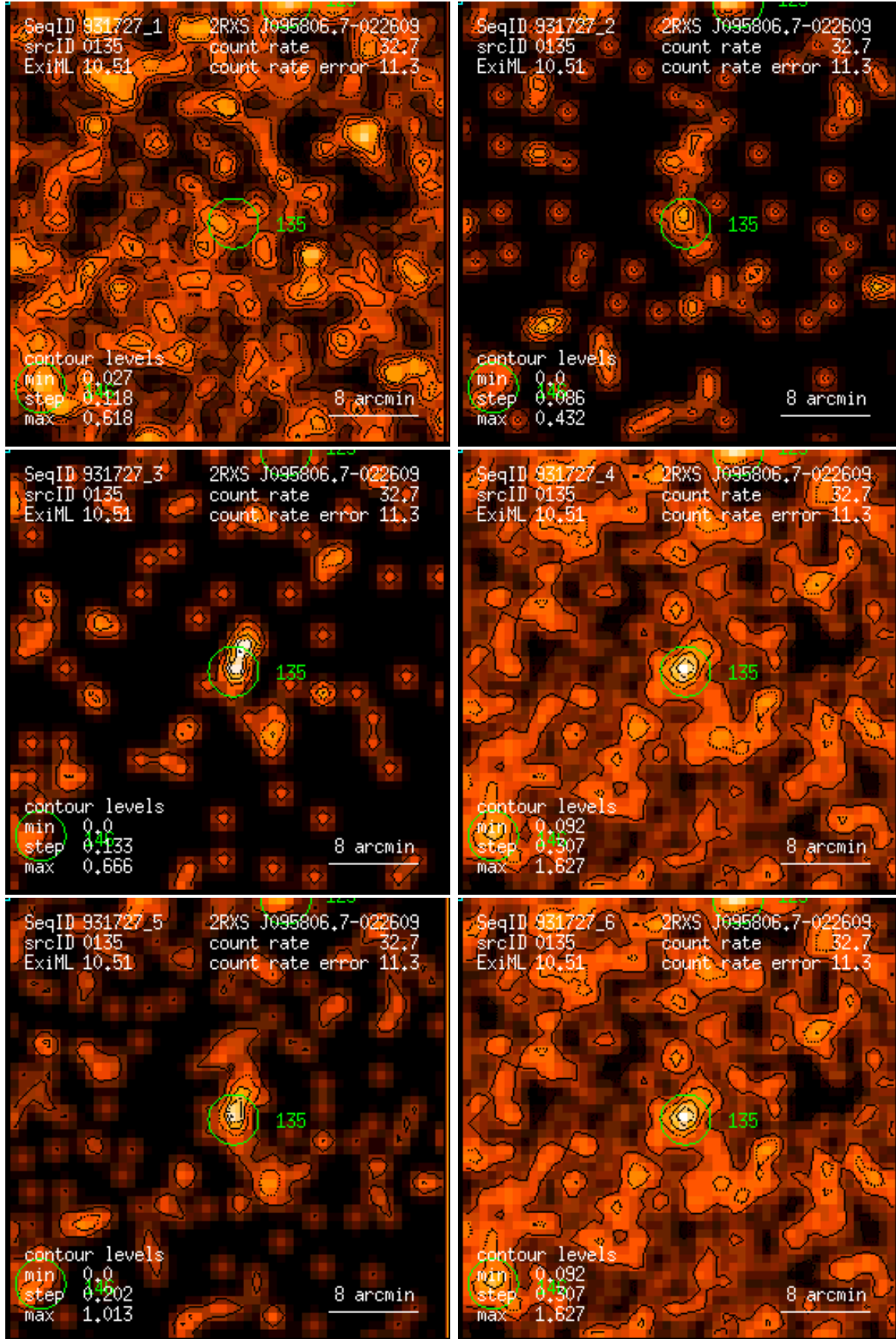
Figure 135: RASS 931727: detection 0135: band rate images, Gaussian filter: (1) PSPC channels 11 – 41, (2) 52 – 90, (3) 91 – 201, (4) 11 – 235, (5) 52 – 201, (6) 11 – 201. Broad band rates in counts/ks. Band rate contour levels in counts/ks/arcmin 2 .
