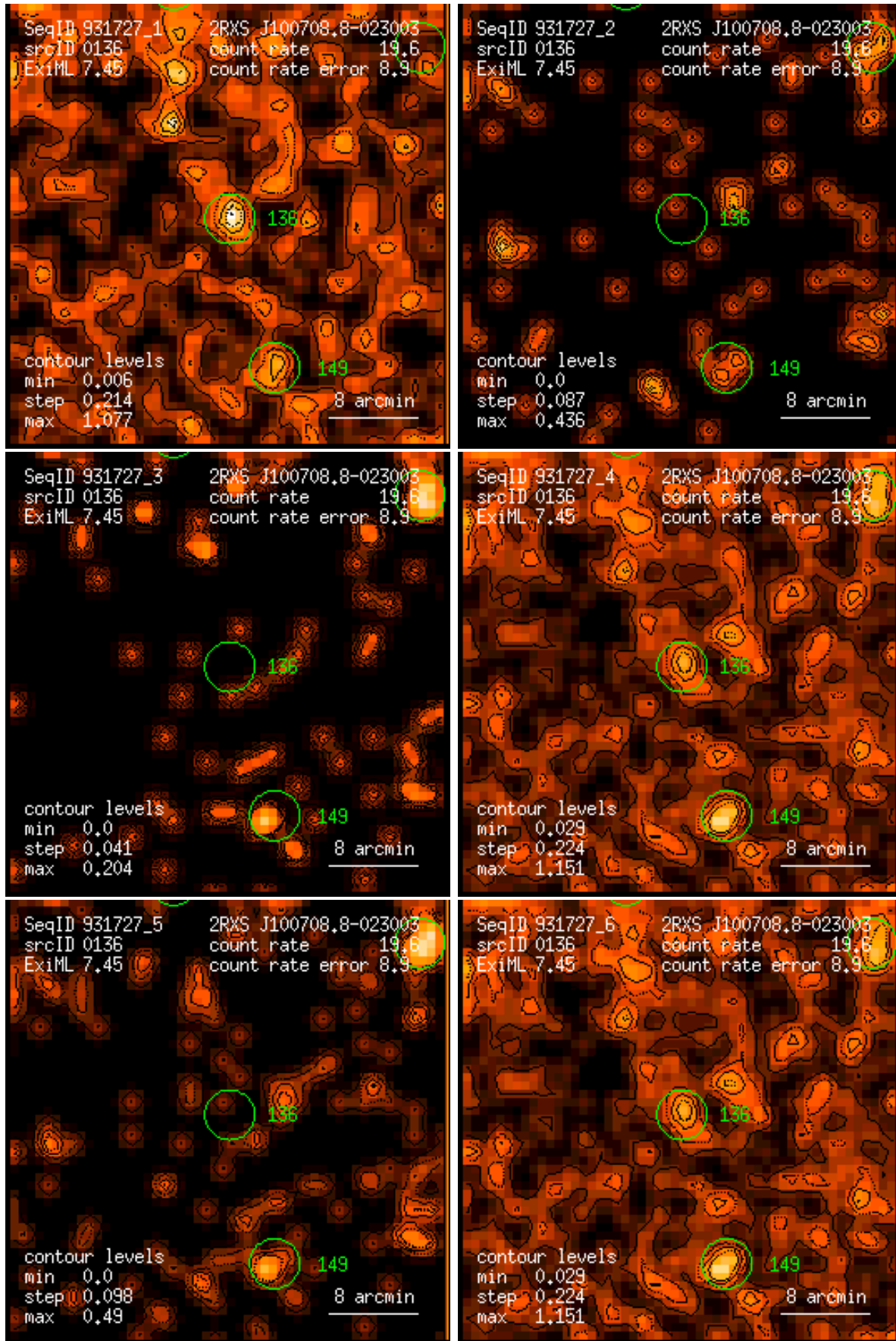
Figure 136: RASS 931727: detection 0136: band rate images, Gaussian filter: (1) PSPC channels 11 – 41, (2) 52 – 90, (3) 91 – 201, (4) 11 – 235, (5) 52 – 201, (6) 11 – 201. Broad band rates in counts/ks. Band rate contour levels in counts/ks/arcmin 2 .
