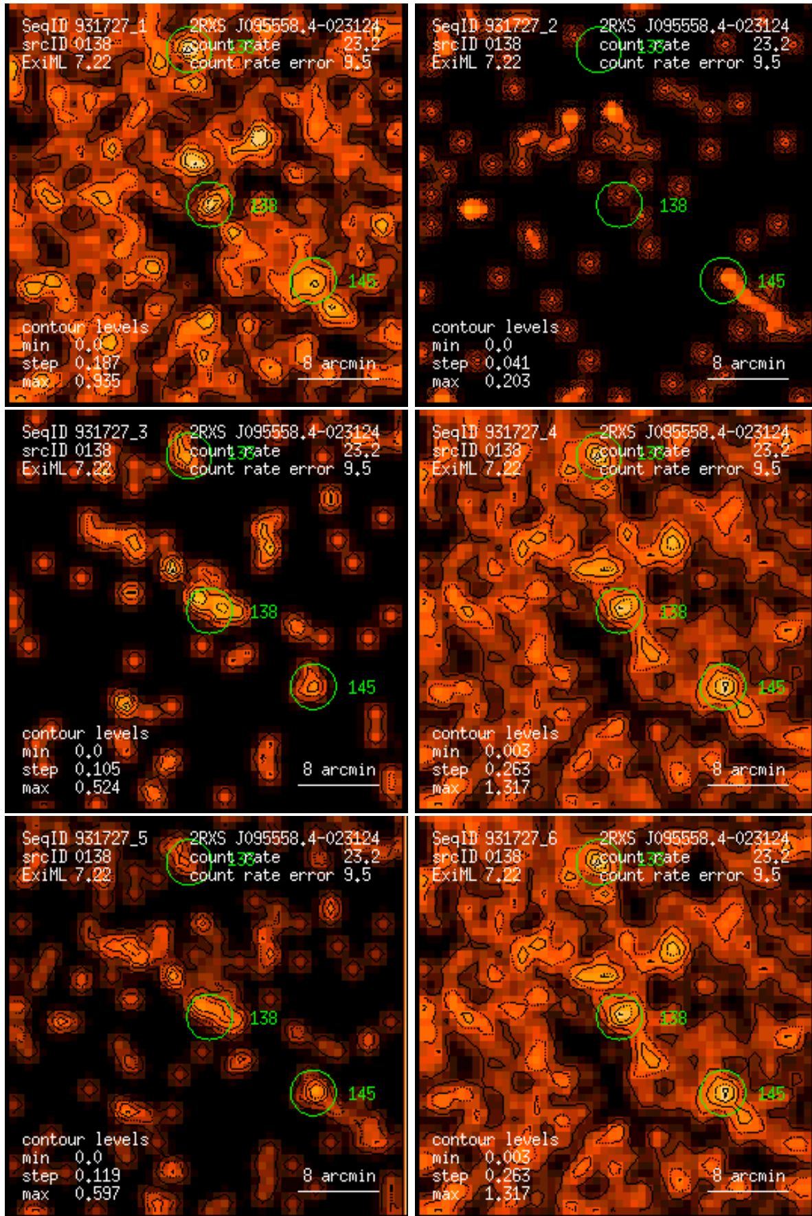
Figure 138: RASS 931727: detection 0138: band rate images, Gaussian filter: (1) PSPC channels 11 – 41, (2) 52 – 90, (3) 91 – 201, (4) 11 – 235, (5) 52 – 201, (6) 11 – 201. Broad band rates in counts/ks. Band rate contour levels in counts/ks/arcmin 2 .
