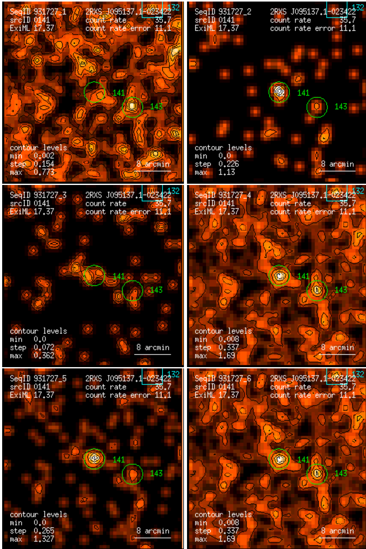
Figure 141: RASS 931727: detection 0141: band rate images, Gaussian filter: (1) PSPC channels 11 – 41, (2) 52 – 90, (3) 91 – 201, (4) 11 – 235, (5) 52 – 201, (6) 11 – 201. Broad band rates in counts/ks. Band rate contour levels in counts/ks/arcmin 2 .
