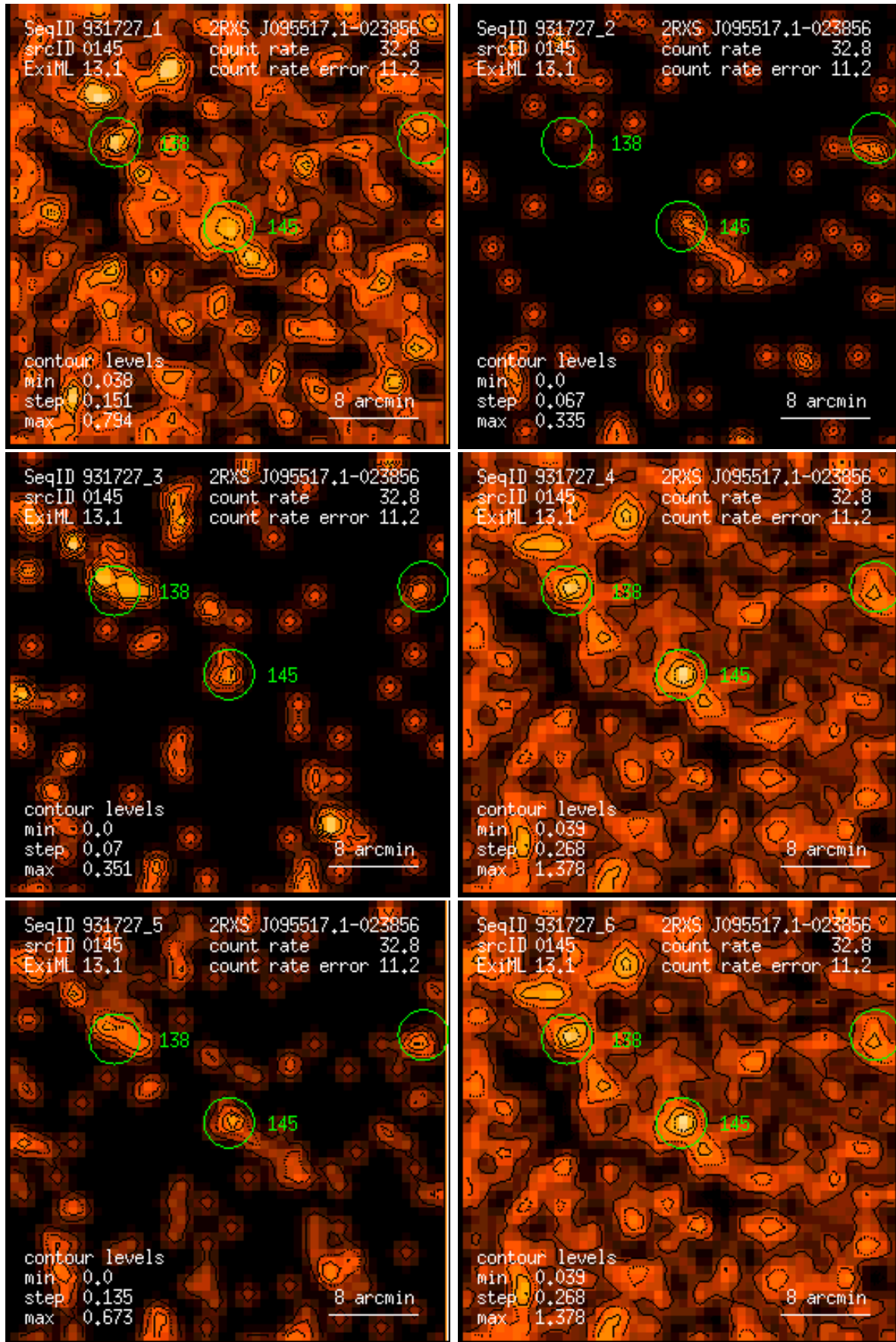
Figure 145: RASS 931727: detection 0145: band rate images, Gaussian filter: (1) PSPC channels 11 – 41, (2) 52 – 90, (3) 91 – 201, (4) 11 – 235, (5) 52 – 201, (6) 11 – 201. Broad band rates in counts/ks. Band rate contour levels in counts/ks/arcmin 2 .
