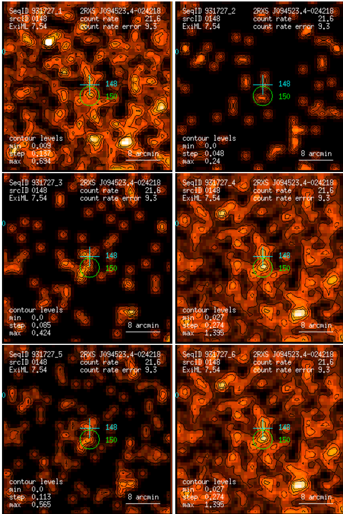
Figure 148: RASS 931727: detection 0148: band rate images, Gaussian filter: (1) PSPC channels 11 – 41, (2) 52 – 90, (3) 91 – 201, (4) 11 – 235, (5) 52 – 201, (6) 11 – 201. Broad band rates in counts/ks. Band rate contour levels in counts/ks/arcmin 2 .
