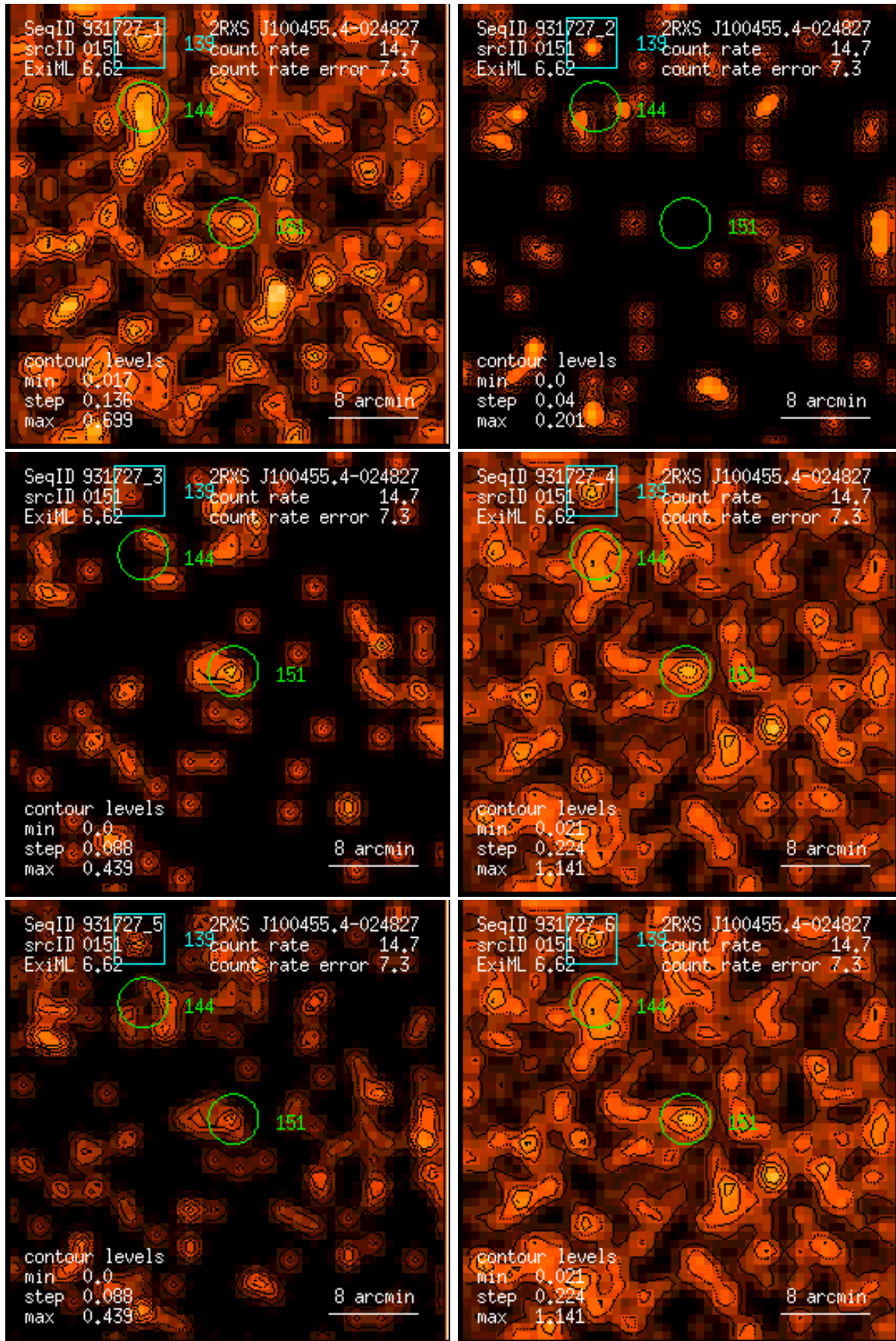
Figure 151: RASS 931727: detection 0151: band rate images, Gaussian filter: (1) PSPC channels 11 – 41, (2) 52 – 90, (3) 91 – 201, (4) 11 – 235, (5) 52 – 201, (6) 11 – 201. Broad band rates in counts/ks. Band rate contour levels in counts/ks/arcmin 2 .
