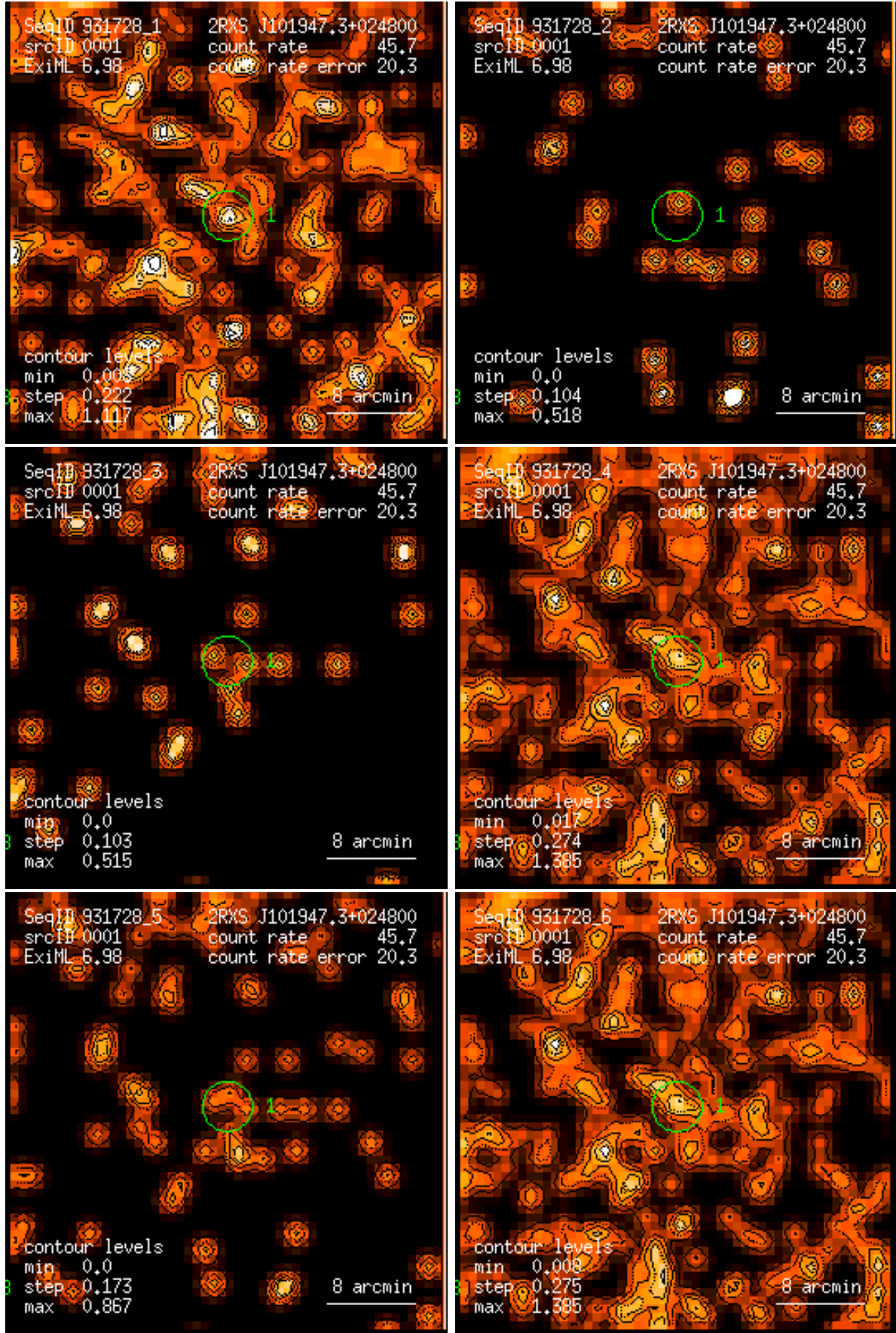
Figure 1: RASS 931728: detection 0001: band rate images, Gaussian filter: (1) PSPC channels 11 – 41, (2) 52 – 90, (3) 91 – 201, (4) 11 – 235, (5) 52 – 201, (6) 11 – 201. Broad band rates in counts/ks. Band rate contour levels in counts/ks/arcmin 2 .
