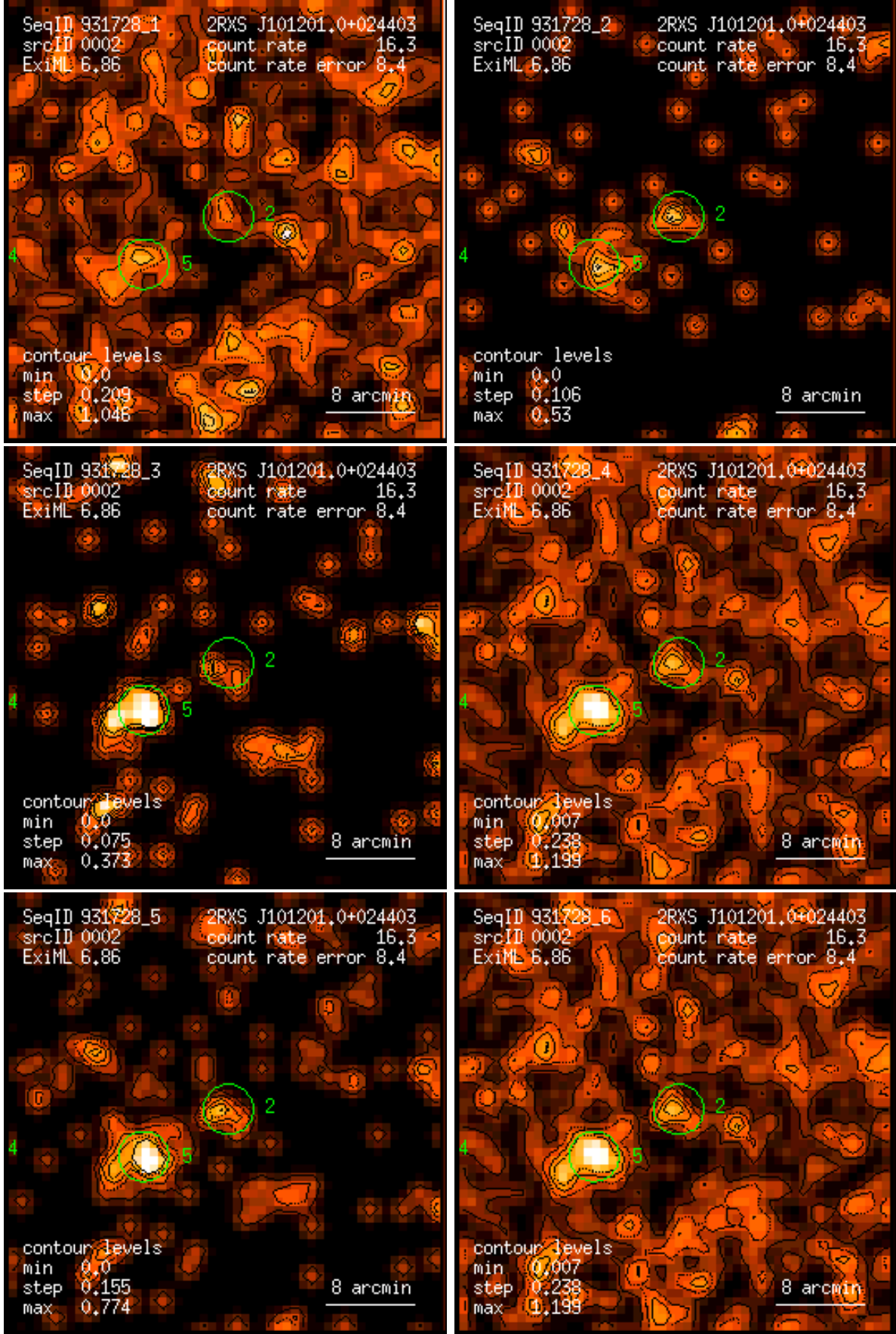
Figure 2: RASS 931728: detection 0002: band rate images, Gaussian filter: (1) PSPC channels 11 – 41, (2) 52 – 90, (3) 91 – 201, (4) 11 – 235, (5) 52 – 201, (6) 11 – 201. Broad band rates in counts/ks. Band rate contour levels in counts/ks/arcmin 2 .
