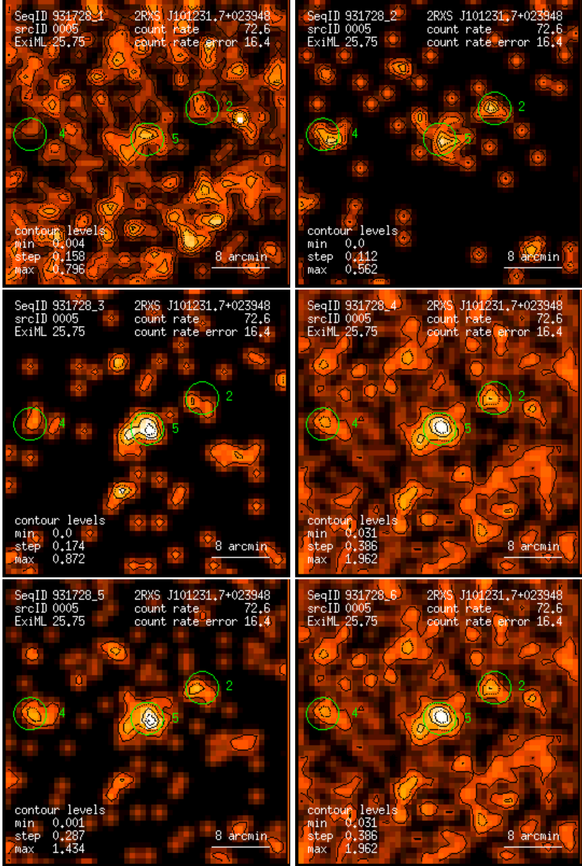
Figure 5: RASS 931728: detection 0005: band rate images, Gaussian filter: (1) PSPC channels 11 – 41, (2) 52 – 90, (3) 91 – 201, (4) 11 – 235, (5) 52 – 201, (6) 11 – 201. Broad band rates in counts/ks. Band rate contour levels in counts/ks/arcmin 2 .
