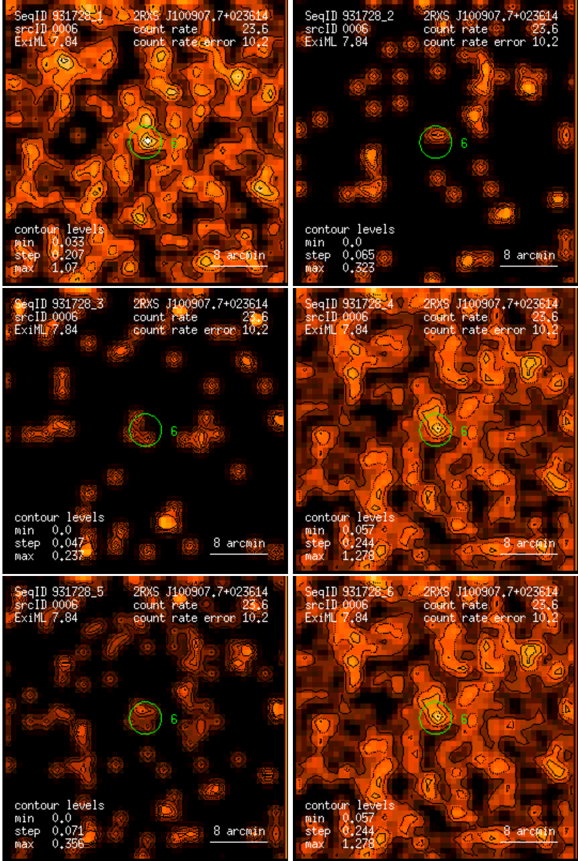
Figure 6: RASS 931728: detection 0006: band rate images, Gaussian filter: (1) PSPC channels 11 – 41, (2) 52 – 90, (3) 91 – 201, (4) 11 – 235, (5) 52 – 201, (6) 11 – 201. Broad band rates in counts/ks. Band rate contour levels in counts/ks/arcmin 2 .
