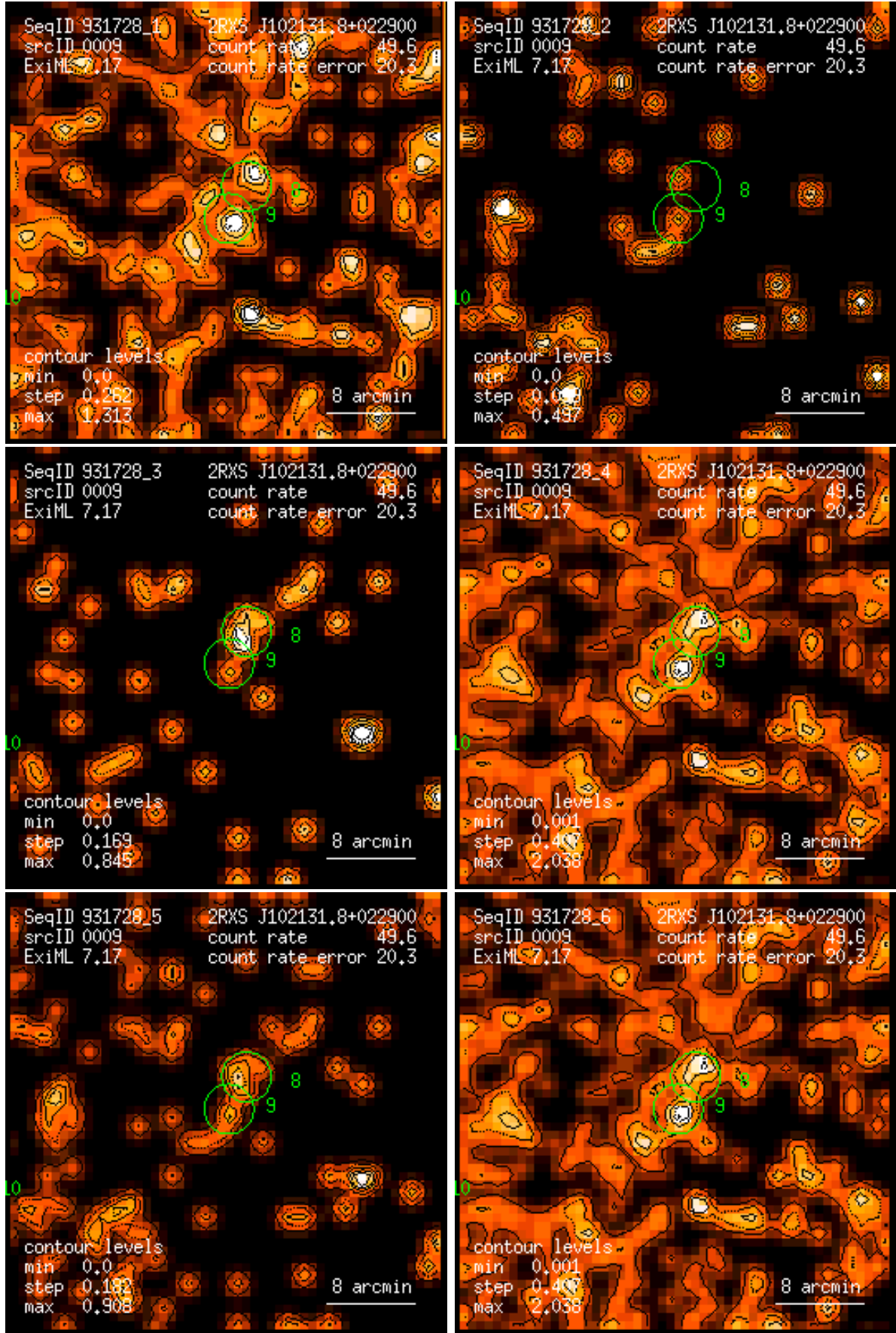
Figure 9: RASS 931728: detection 0009: band rate images, Gaussian filter: (1) PSPC channels 11 – 41, (2) 52 – 90, (3) 91 – 201, (4) 11 – 235, (5) 52 – 201, (6) 11 – 201. Broad band rates in counts/ks. Band rate contour levels in counts/ks/arcmin 2 .
