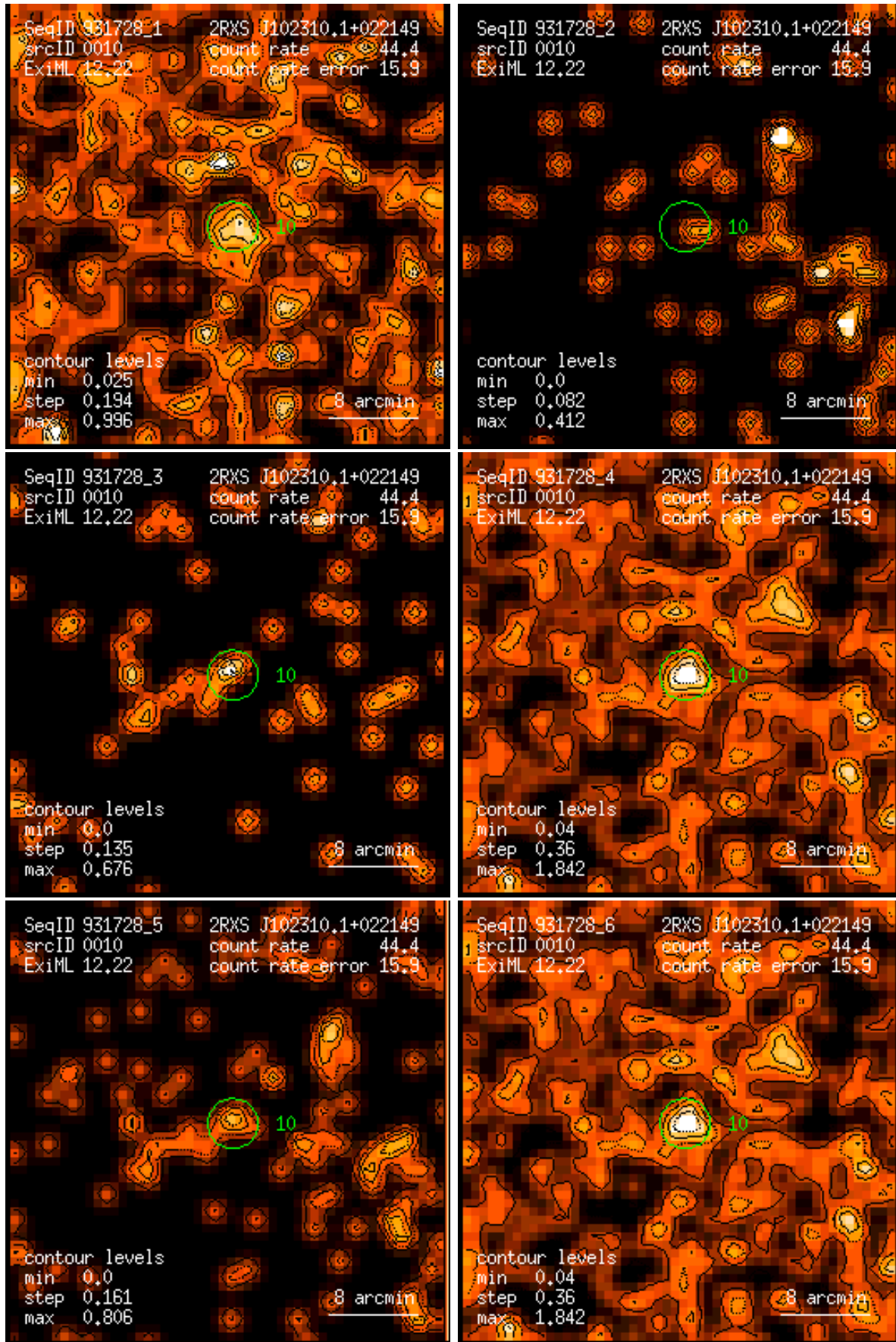
Figure 10: RASS 931728: detection 0010: band rate images, Gaussian filter: (1) PSPC channels 11 – 41, (2) 52 – 90, (3) 91 – 201, (4) 11 – 235, (5) 52 – 201, (6) 11 – 201. Broad band rates in counts/ks. Band rate contour levels in counts/ks/arcmin 2 .
