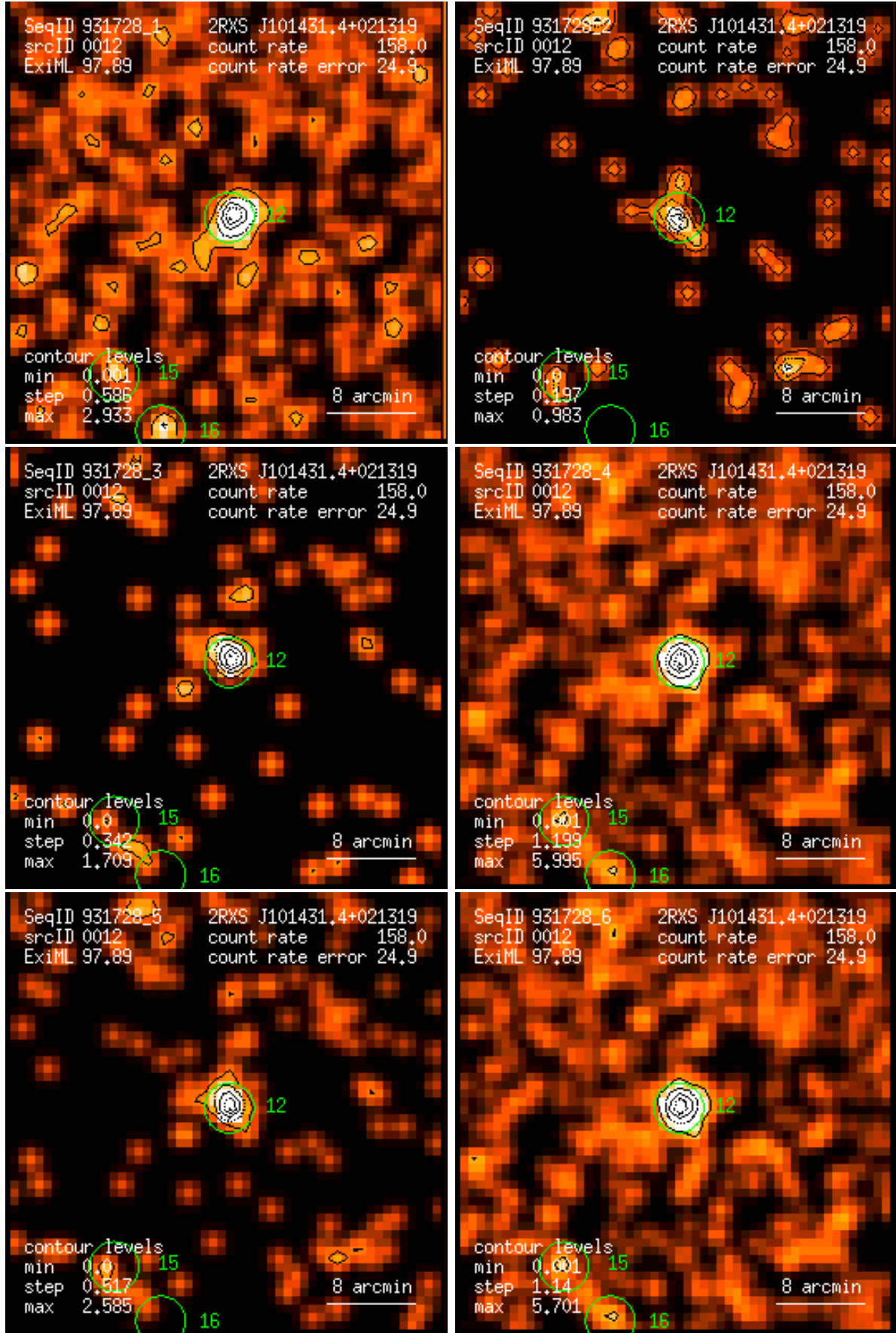
Figure 12: RASS 931728: detection 0012: band rate images, Gaussian filter: (1) PSPC channels 11 – 41, (2) 52 – 90, (3) 91 – 201, (4) 11 – 235, (5) 52 – 201, (6) 11 – 201. Broad band rates in counts/ks. Band rate contour levels in counts/ks/arcmin 2 .
