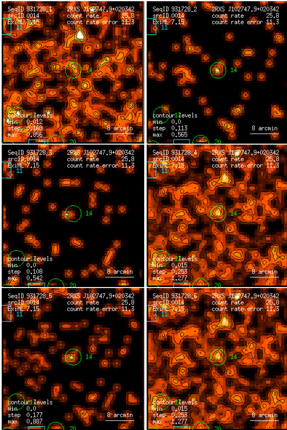
Figure 14: RASS 931728: detection 0014: band rate images, Gaussian filter: (1) PSPC channels 11 – 41, (2) 52 – 90, (3) 91 – 201, (4) 11 – 235, (5) 52 – 201, (6) 11 – 201. Broad band rates in counts/ks. Band rate contour levels in counts/ks/arcmin 2 .
