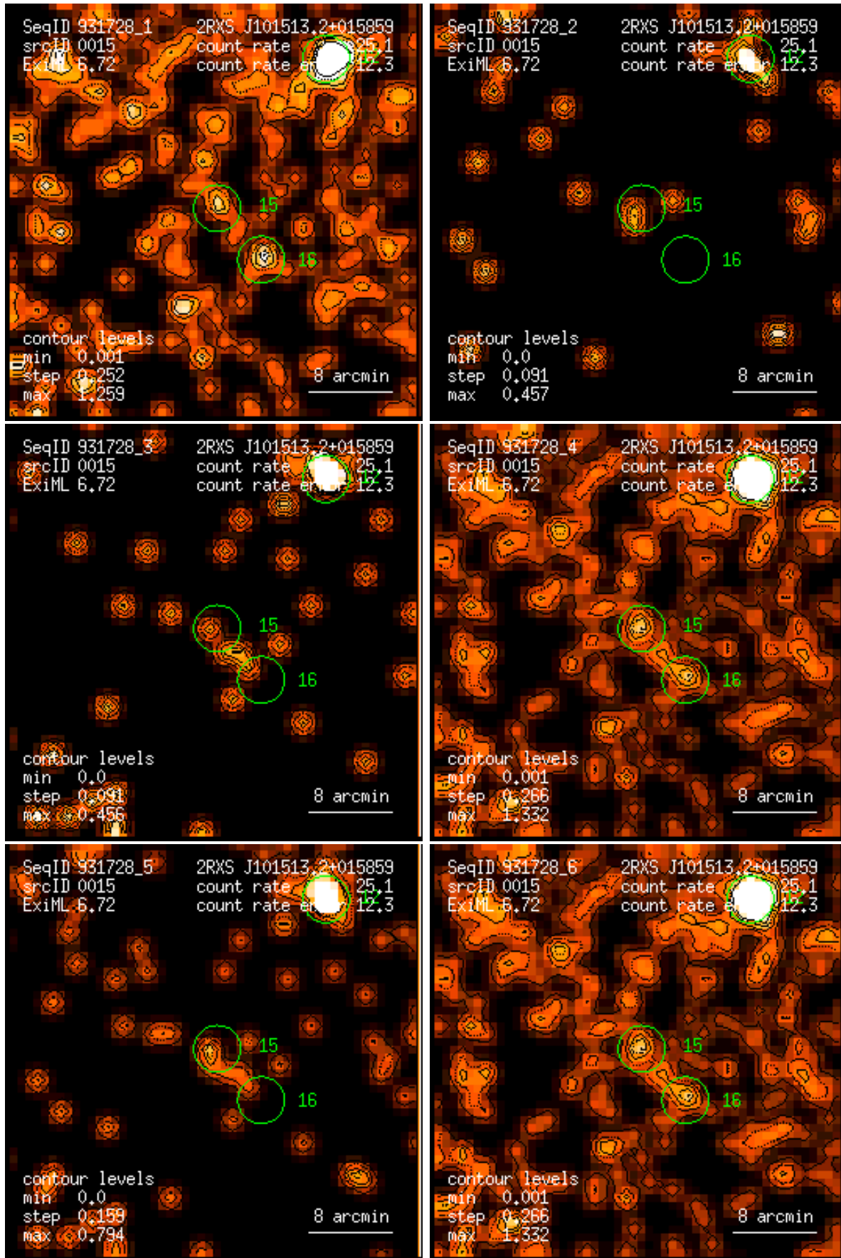
Figure 15: RASS 931728: detection 0015: band rate images, Gaussian filter: (1) PSPC channels 11 – 41, (2) 52 – 90, (3) 91 – 201, (4) 11 – 235, (5) 52 – 201, (6) 11 – 201. Broad band rates in counts/ks. Band rate contour levels in counts/ks/arcmin 2 .
