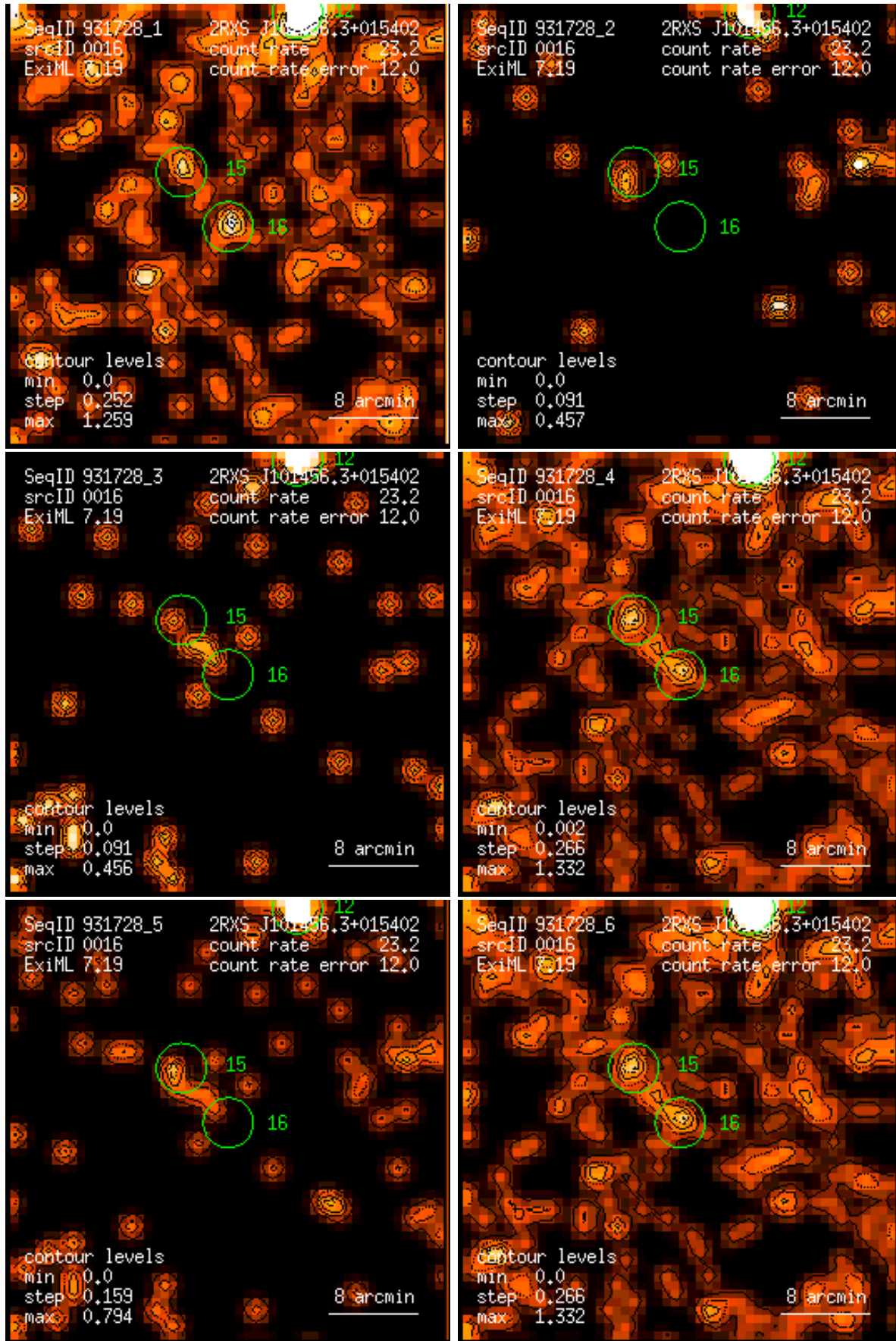
Figure 16: RASS 931728: detection 0016: band rate images, Gaussian filter: (1) PSPC channels 11 – 41, (2) 52 – 90, (3) 91 – 201, (4) 11 – 235, (5) 52 – 201, (6) 11 – 201. Broad band rates in counts/ks. Band rate contour levels in counts/ks/arcmin 2 .
