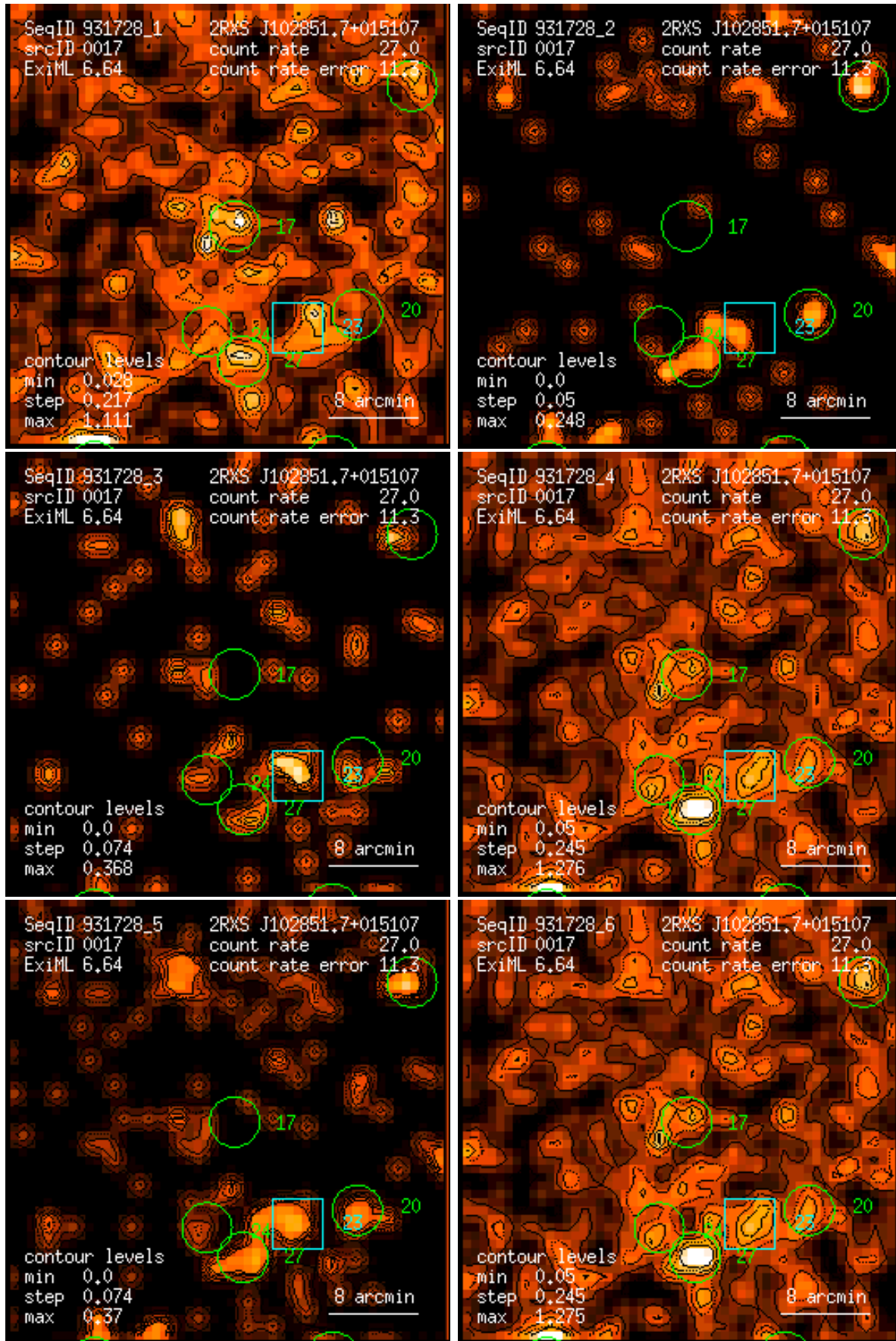
Figure 17: RASS 931728: detection 0017: band rate images, Gaussian filter: (1) PSPC channels 11 – 41, (2) 52 – 90, (3) 91 – 201, (4) 11 – 235, (5) 52 – 201, (6) 11 – 201. Broad band rates in counts/ks. Band rate contour levels in counts/ks/arcmin 2 .
