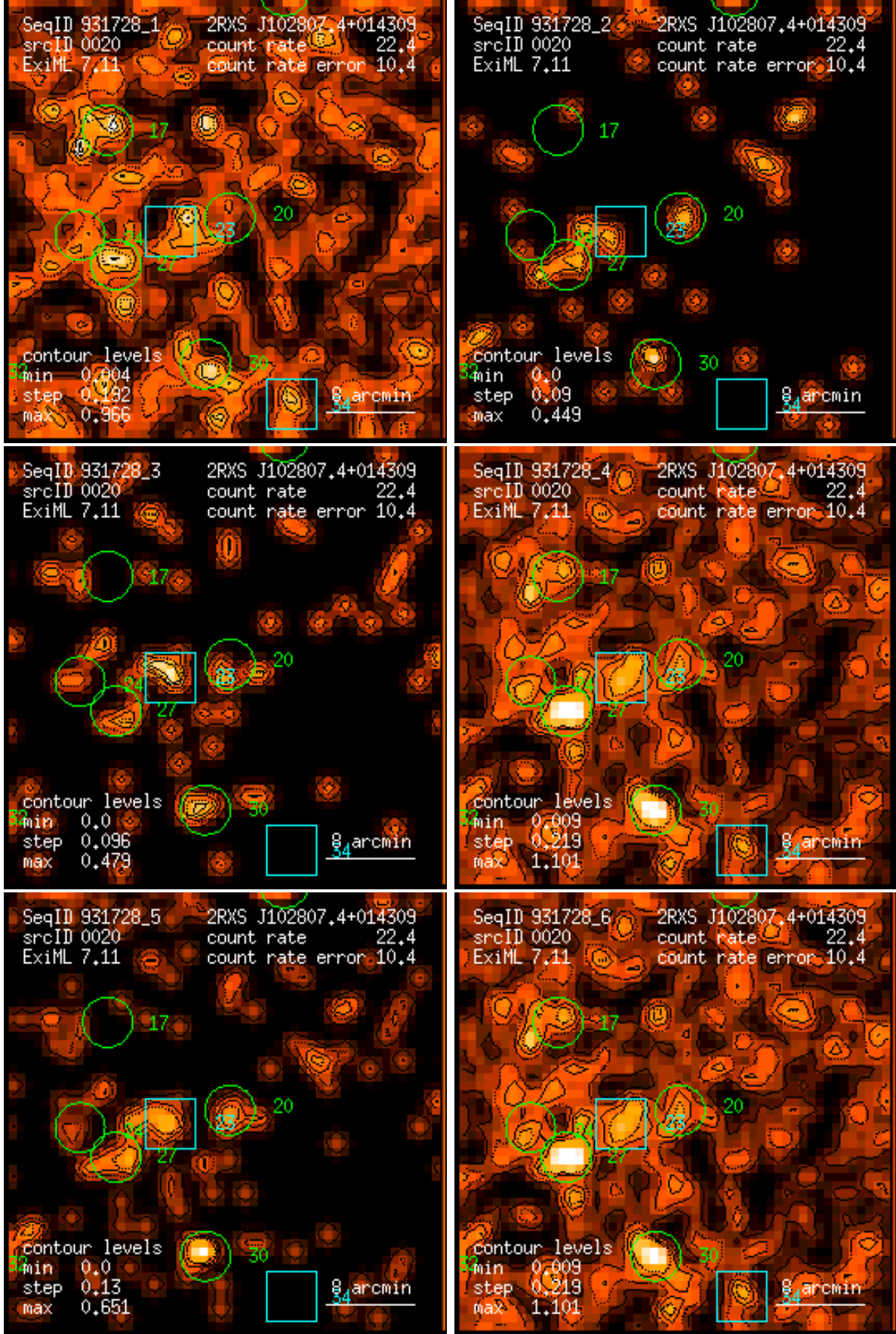
Figure 20: RASS 931728: detection 0020: band rate images, Gaussian filter: (1) PSPC channels 11 – 41, (2) 52 – 90, (3) 91 – 201, (4) 11 – 235, (5) 52 – 201, (6) 11 – 201. Broad band rates in counts/ks. Band rate contour levels in counts/ks/arcmin 2 .
