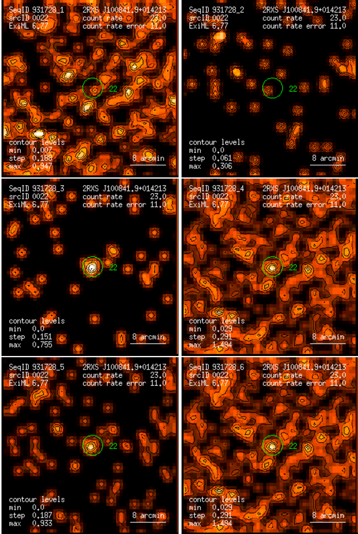
Figure 22: RASS 931728: detection 0022: band rate images, Gaussian filter: (1) PSPC channels 11 – 41, (2) 52 – 90, (3) 91 – 201, (4) 11 – 235, (5) 52 – 201, (6) 11 – 201. Broad band rates in counts/ks. Band rate contour levels in counts/ks/arcmin 2 .
