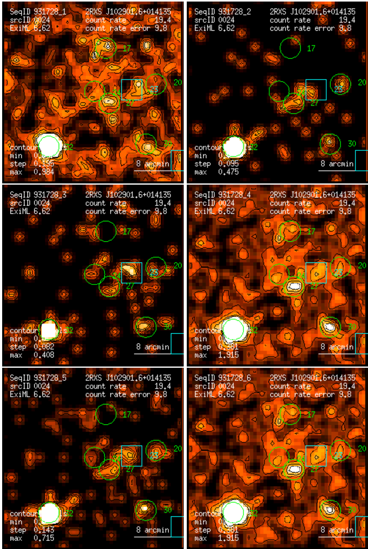
Figure 24: RASS 931728: detection 0024: band rate images, Gaussian filter: (1) PSPC channels 11 – 41, (2) 52 – 90, (3) 91 – 201, (4) 11 – 235, (5) 52 – 201, (6) 11 – 201. Broad band rates in counts/ks. Band rate contour levels in counts/ks/arcmin 2 .
