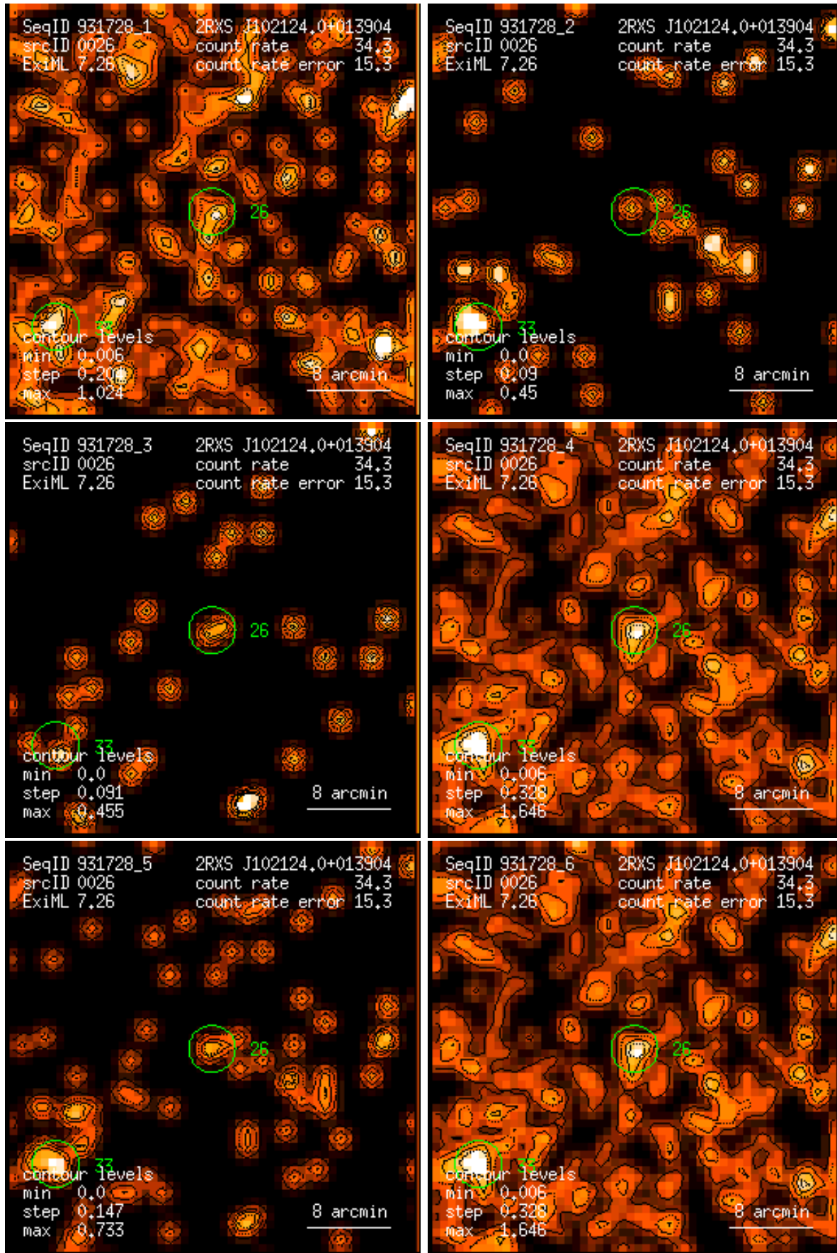
Figure 26: RASS 931728: detection 0026: band rate images, Gaussian filter: (1) PSPC channels 11 – 41, (2) 52 – 90, (3) 91 – 201, (4) 11 – 235, (5) 52 – 201, (6) 11 – 201. Broad band rates in counts/ks. Band rate contour levels in counts/ks/arcmin 2 .
