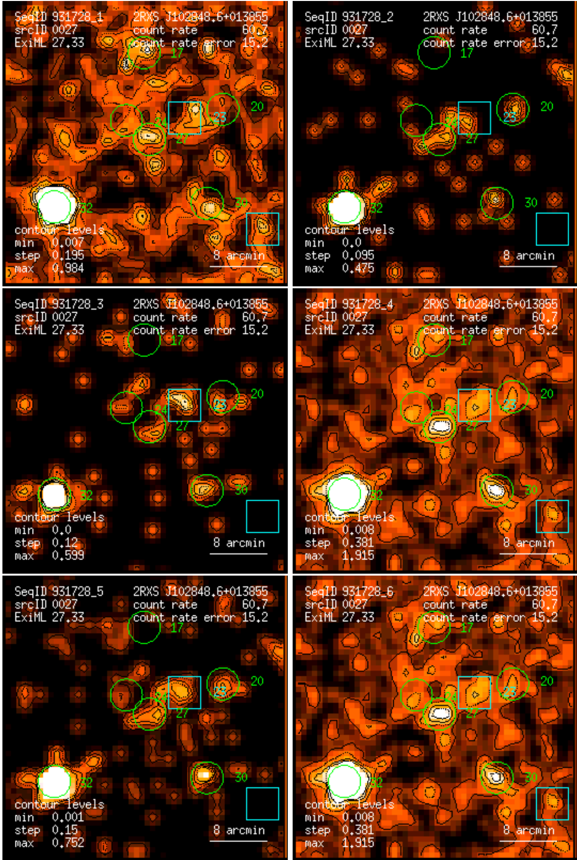
Figure 27: RASS 931728: detection 0027: band rate images, Gaussian filter: (1) PSPC channels 11 – 41, (2) 52 – 90, (3) 91 – 201, (4) 11 – 235, (5) 52 – 201, (6) 11 – 201. Broad band rates in counts/ks. Band rate contour levels in counts/ks/arcmin 2 .
