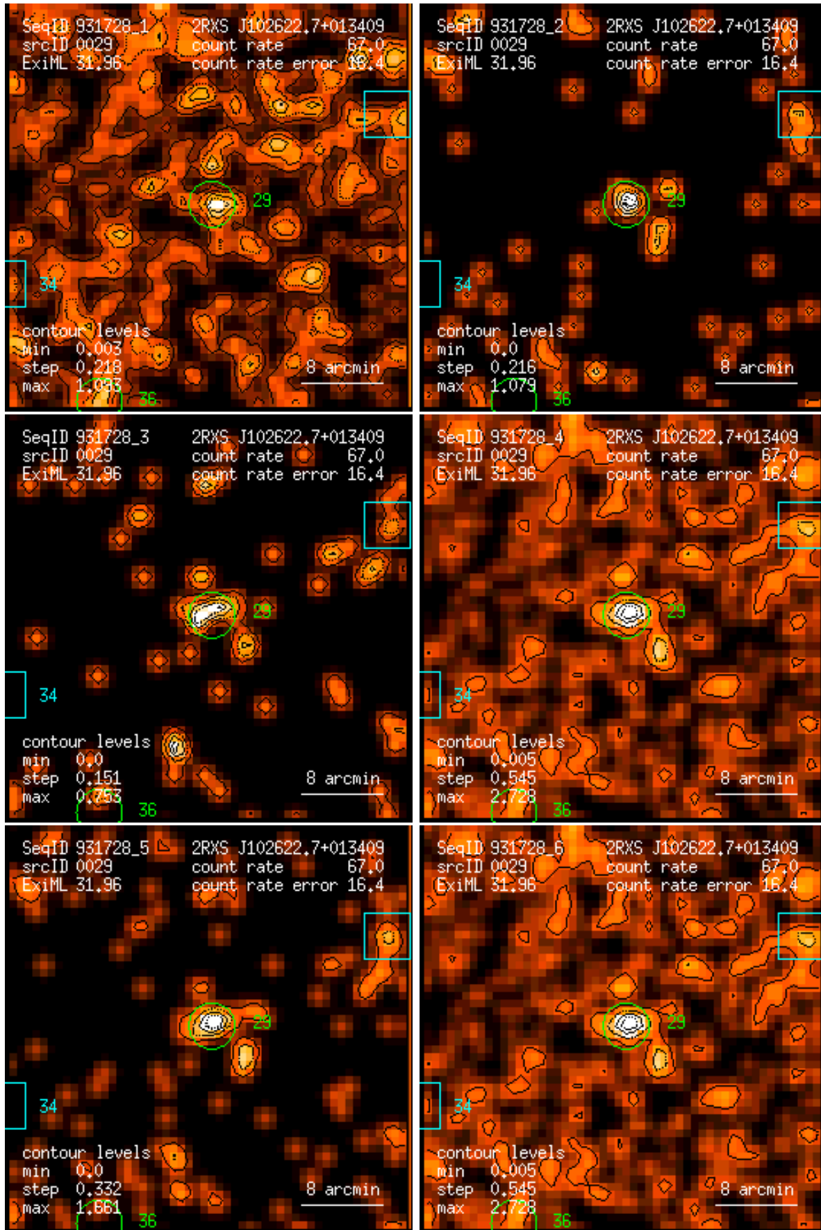
Figure 29: RASS 931728: detection 0029: band rate images, Gaussian filter: (1) PSPC channels 11 – 41, (2) 52 – 90, (3) 91 – 201, (4) 11 – 235, (5) 52 – 201, (6) 11 – 201. Broad band rates in counts/ks. Band rate contour levels in counts/ks/arcmin 2 .
