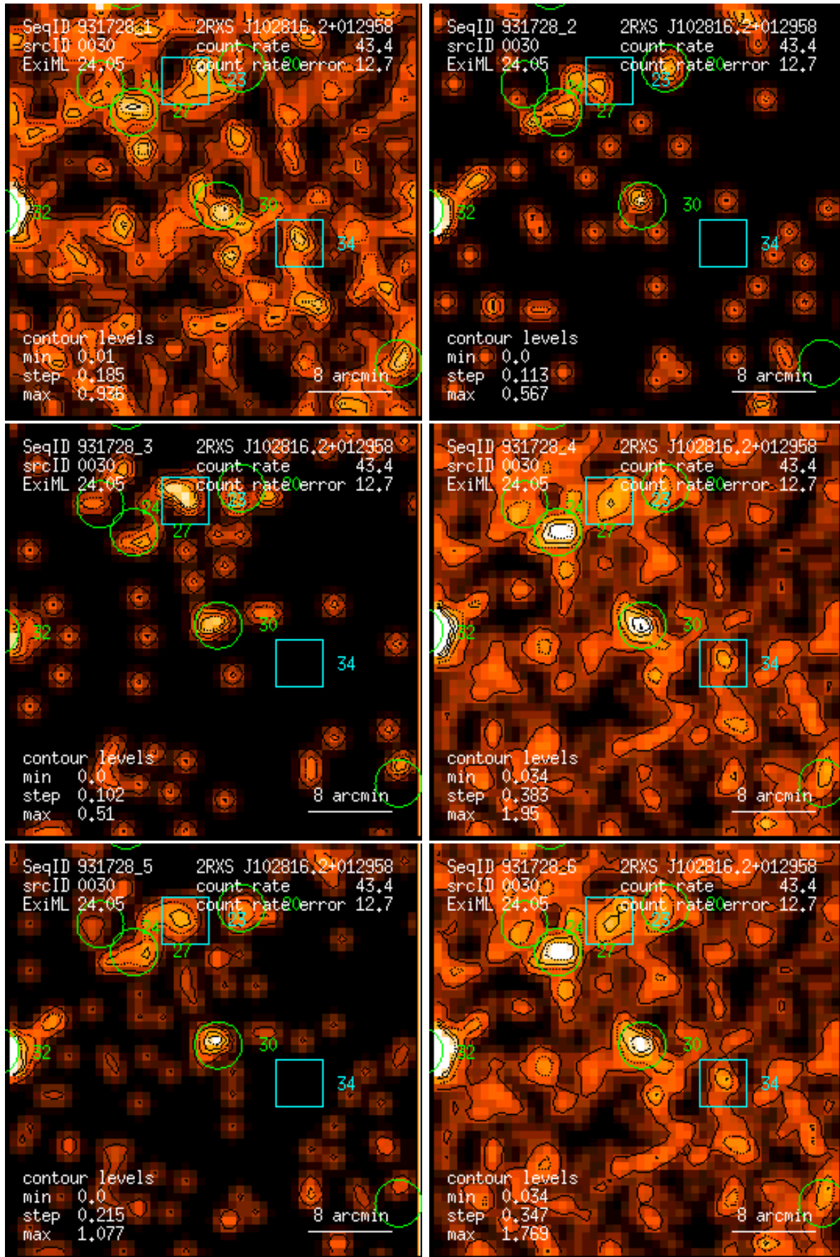
Figure 30: RASS 931728: detection 0030: band rate images, Gaussian filter: (1) PSPC channels 11 – 41, (2) 52 – 90, (3) 91 – 201, (4) 11 – 235, (5) 52 – 201, (6) 11 – 201. Broad band rates in counts/ks. Band rate contour levels in counts/ks/arcmin 2 .
