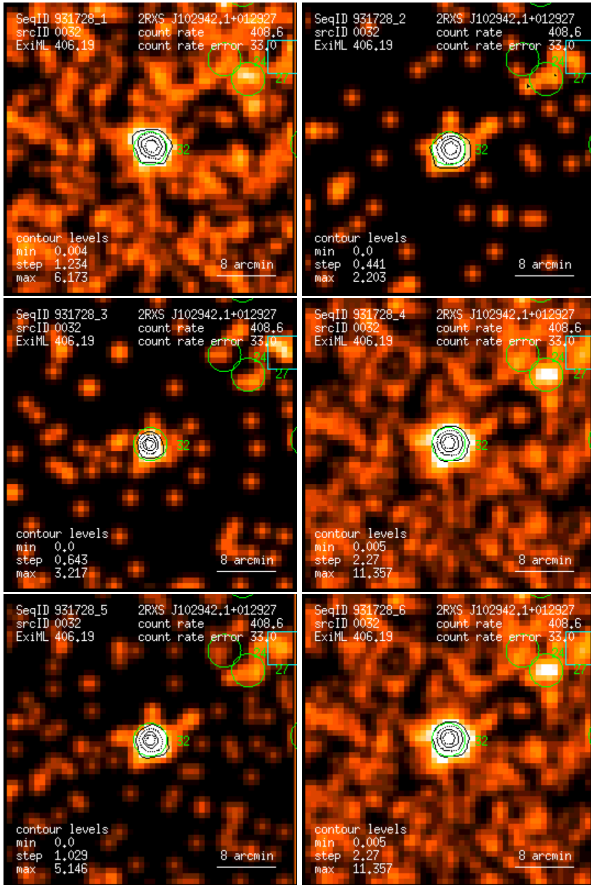
Figure 32: RASS 931728: detection 0032: band rate images, Gaussian filter: (1) PSPC channels 11 – 41, (2) 52 – 90, (3) 91 – 201, (4) 11 – 235, (5) 52 – 201, (6) 11 – 201. Broad band rates in counts/ks. Band rate contour levels in counts/ks/arcmin 2 .
