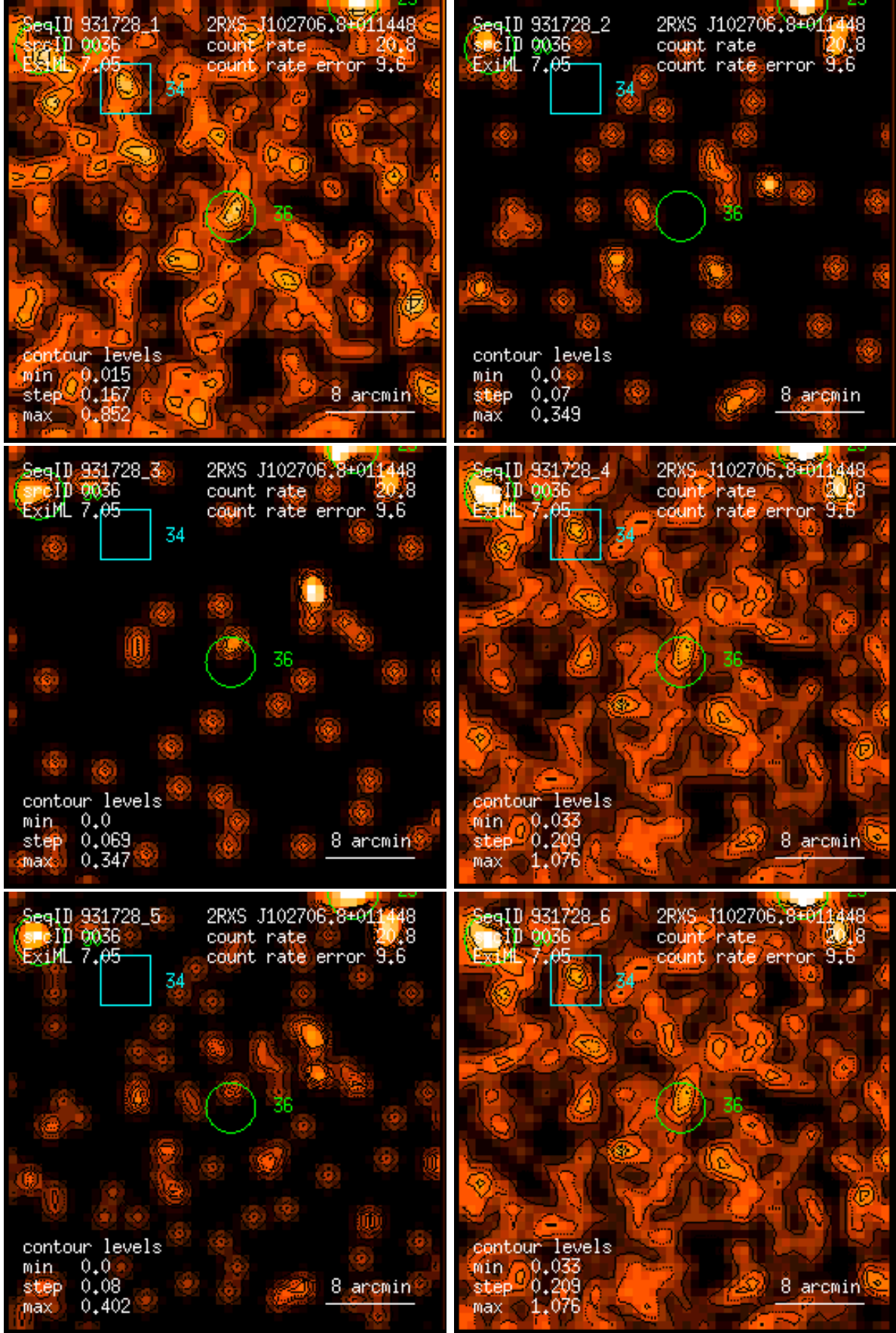
Figure 36: RASS 931728: detection 0036: band rate images, Gaussian filter: (1) PSPC channels 11 – 41, (2) 52 – 90, (3) 91 – 201, (4) 11 – 235, (5) 52 – 201, (6) 11 – 201. Broad band rates in counts/ks. Band rate contour levels in counts/ks/arcmin 2 .
