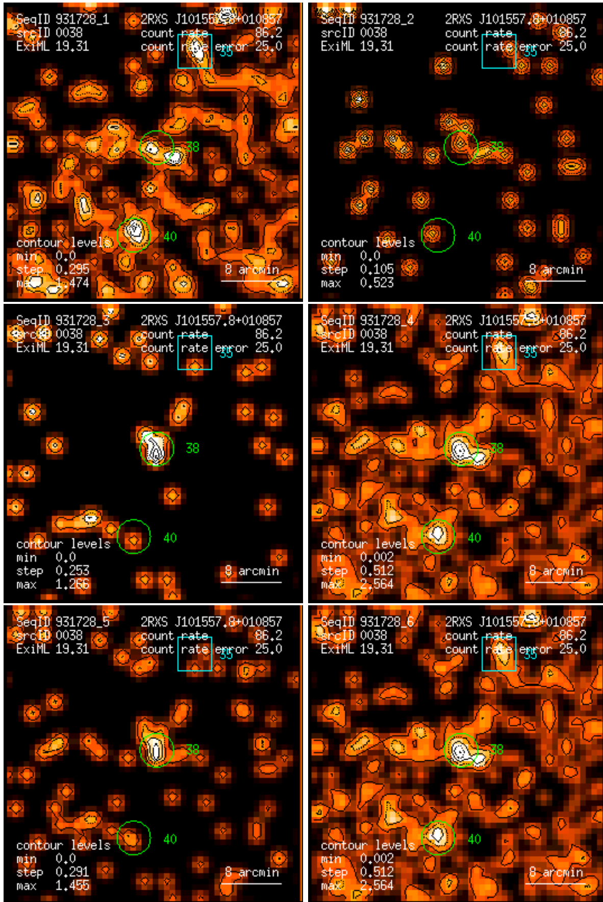
Figure 38: RASS 931728: detection 0038: band rate images, Gaussian filter: (1) PSPC channels 11 – 41, (2) 52 – 90, (3) 91 – 201, (4) 11 – 235, (5) 52 – 201, (6) 11 – 201. Broad band rates in counts/ks. Band rate contour levels in counts/ks/arcmin 2 .
