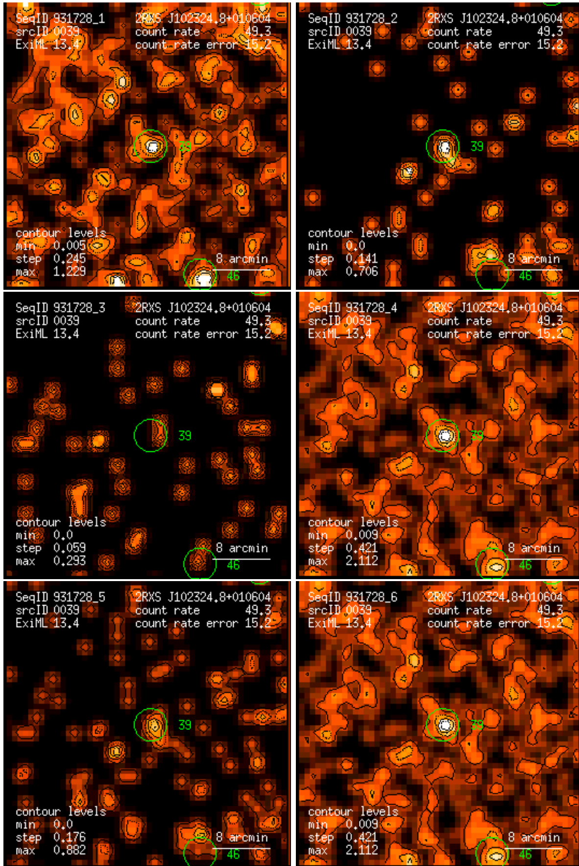
Figure 39: RASS 931728: detection 0039: band rate images, Gaussian filter: (1) PSPC channels 11 – 41, (2) 52 – 90, (3) 91 – 201, (4) 11 – 235, (5) 52 – 201, (6) 11 – 201. Broad band rates in counts/ks. Band rate contour levels in counts/ks/arcmin 2 .
